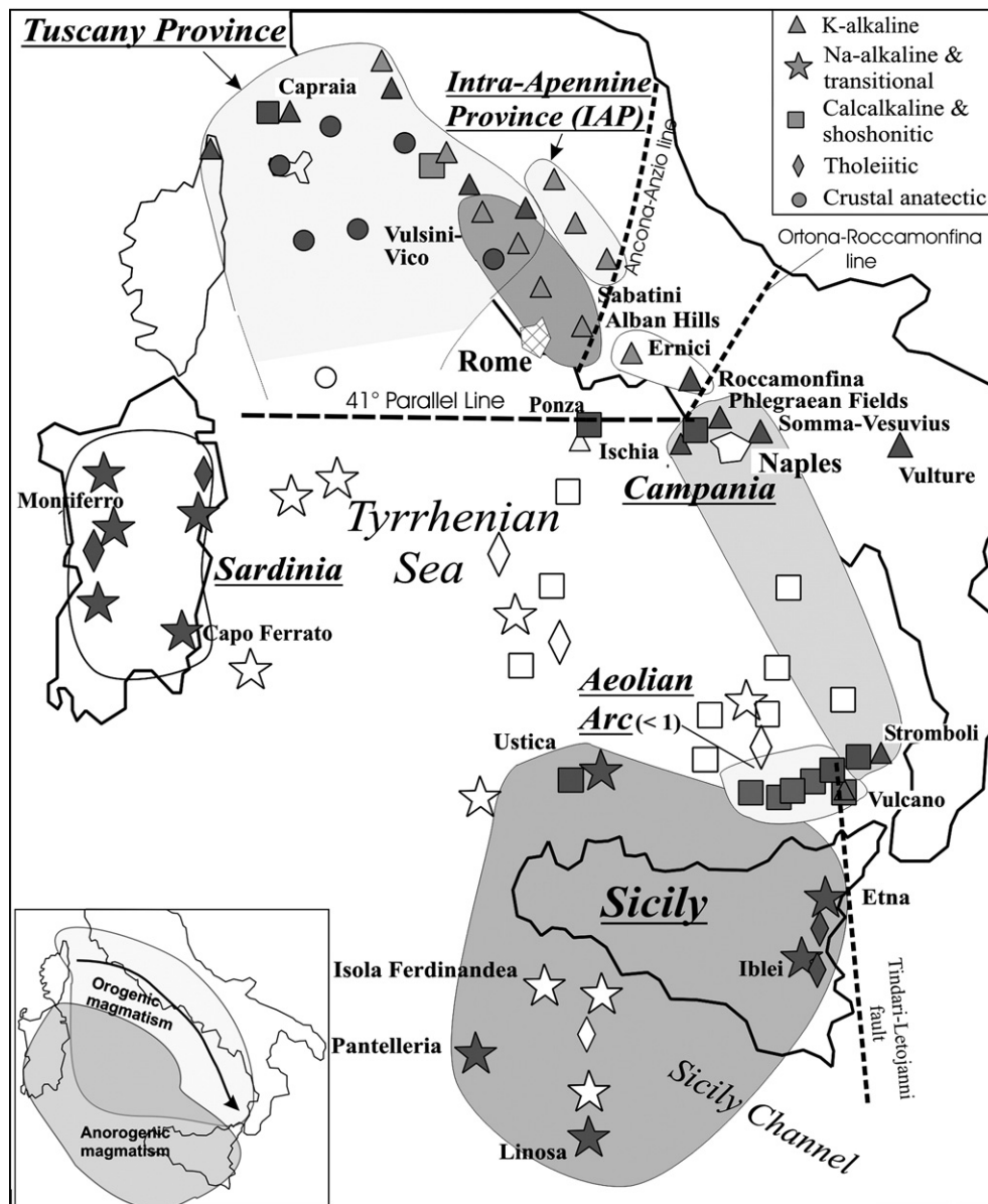
Fig. 12. Plio-Quaternary magmatic provinces in Italy. Modified after Peccherillo (2003) . Inset map shows schematic distribution of orogenic and anorogenic Plio-Quaternary volcanic rocks in the Tyrrhenian area. Arrow in the inset map indicates age variation of orogenic magmatism.
