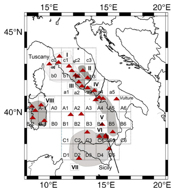
Fig. 13. Magmatic provinces, shown in Fig. 12, superimposed to the grid of the geophysical model. Gray areas represent the main magmatic provinces. I: Tuscany Province; II: Intra-Apennine Province; III: Roman Province; IV: Ernici–Roccamonfina Province; V: Campania–Stromboli; VI: Western–Central Aeolian arc; VII: Sicily Province; VIII: Sardinia. Red triangles represent the different recent and active volcanoes within the study area. (For interpretation of the references to colour in this figure legend, the reader is referred to the web version of this article.)
