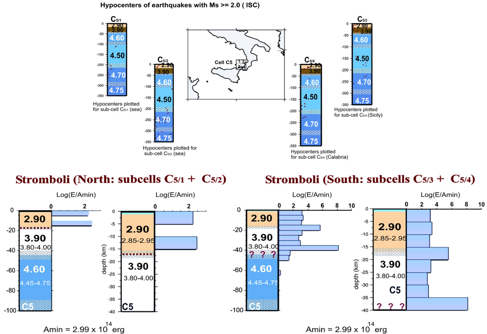
Fig. 7. Seismic energy vs. depth for all events with magnitude above the completeness threshold, defined by means of an exploratory analysis of the Gutenberg–Richter relation of the earthquake catalogue for each cell extracted from the International Seismological Centre (ISC) catalogue. Case of Stromboli: Cell C5 is divided into a northern (sub-cell C_{5/1} +sub-cell C_{5/2} ) and a southern (sub-cell C_{5/3} +sub-cell C_{5/4} ) part in order to highlight the seismicity space distribution and its contribution to the seismic energy as shown in the lower panel. The Moho depth is well defined (red broken line) in the northern part while uncertain (?) in the southern part of cell C5.
