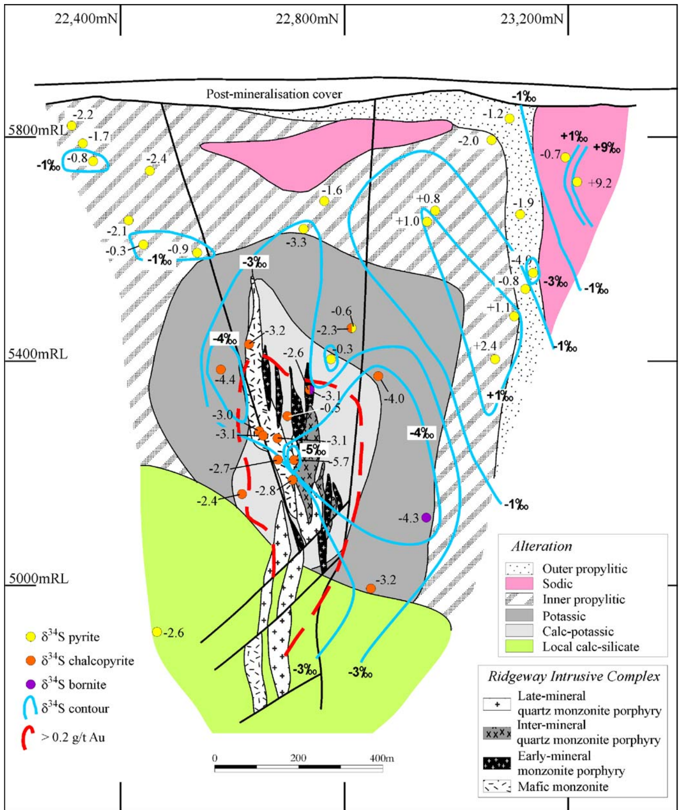
Fig. 7 Contoured values of \delta^{34}\text{S}_{\text{sulfide}} values (per mil) from section 11,050 mE, Ridgeway. Also shown are the locations of the Ridgeway Intrusive Complex, the hydrothermal alteration zones
