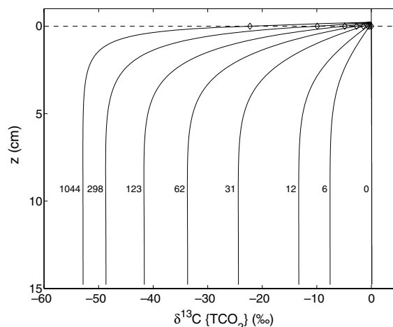
Fig. 12. Model results for porewater \delta^{13}\text{C}_{\text{TCO}_2} as a function of depth and AOM rates (from 0 to 1044 \mu\text{mol cm}^{-2} \text{ y}^{-1} ) at \delta^{13}\text{C}_{\text{CH}_4} = -60\text{‰} . Diamonds indicate model values at the sediment–water interface.
