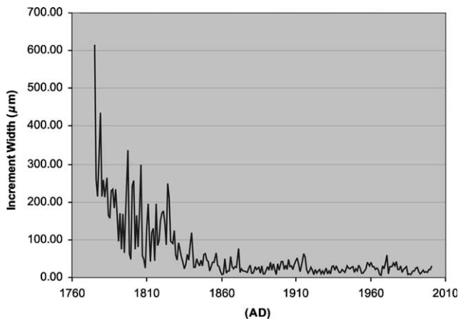
Figure 3 Untreated growth band series from longest-lived live collected shell 010036 (211 years) collected from Fladen Ground in 2001 (RV Scotia trawl s01 189, 58°47.24'N, 0°20.48'E, 125 m water depth)
