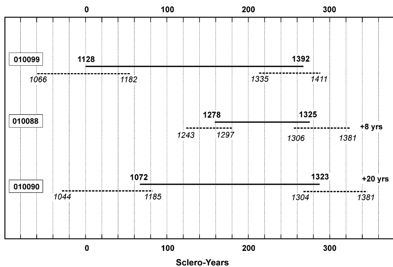
Figure 6 Length of annual series (sclero-years) of shells 010099, 010088 and 010090 plotted by cross-matched best-lagged correlation fits with reservoir-corrected calibrated ages and 1σ errors (ages (bold) and error bars (dashed) calibrated using the intercept method on the marine calibration curve)
