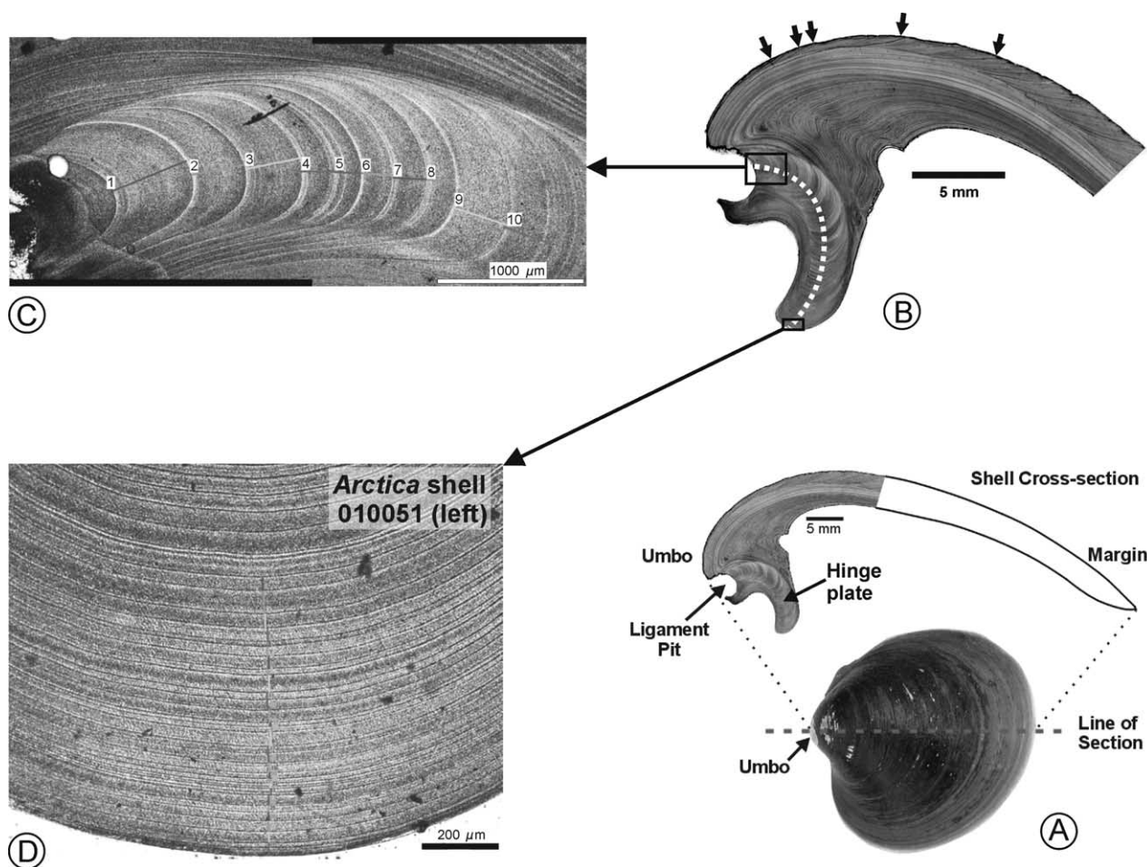
Figure 2 (A) External valve face, showing line of section through Arctica valve used to generate acetate peel replicas. (B) Acetate peel replica cross-section of valve showing annual growth band increments along shell margin (arrows) and within the hinge plate. The axis of growth through the hinge plate used to generate increment data is indicated by the dashed white line. (C) Numbered annual growth bands are measured from the earliest growth bands to the most recent along the axis of growth. Juvenile early bands are wide and reflect the ontogenetic growth curve of the individual (Figure 3). (D) Narrow senescent late bands from the outer part of the hinge plate axis. Youngest increment at base
