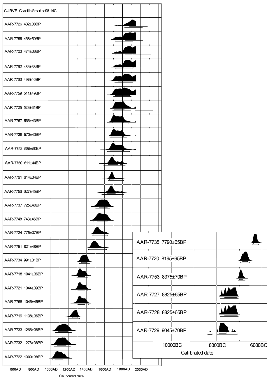
Figure 7 Calibration plot of all age-sorted ^{14}\text{C} dated A. islandica valves with positive reservoir corrected age from the Fladen Ground, northern North Sea showing probability distributions using the marine model (Stuiver et al. , 1998)
