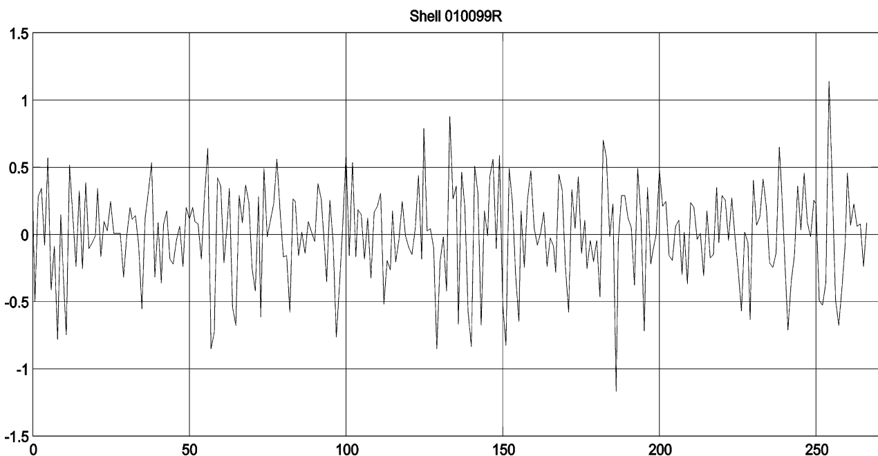
Figure 4 Normalized shell growth plot for longest-lived shell 010099 (267 years) on arbitrary annual timescale; this shell was collected dead. A logarithmic function (unique to each individual) is first applied to the raw data series; the data are then normalized and the residuals from a 15-yr spline calculated producing a standard shell growth plot
