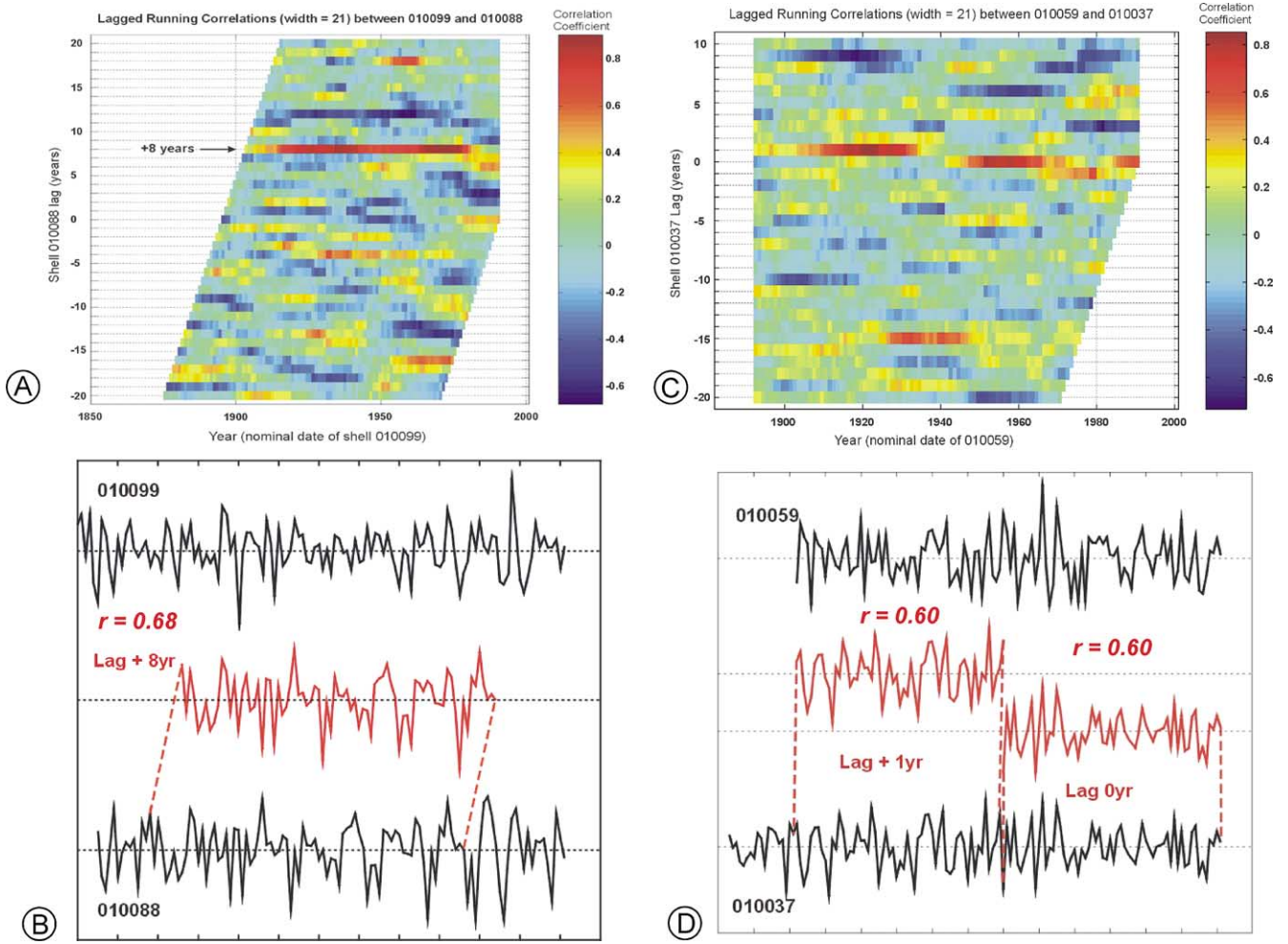
Figure 5 SHELLCORR graphical output showing lagged running correlations (window width = 21) between growth band series. High positive correlations in red, high negative correlations in blue. (A) Correlation between shells 010088 and 010099 showing best and longest correlation at 8-yr lag. Other high correlations (negative and positive) do appear for other lags but these are neither as strong, nor do they persist for as long, as the 8-yr position. (B) The correlation between the normalized shell growth series for shells 010088 and 010099. The best correlation of +0.68 is achieved if series 010088 is moved forwards by 8 years. (C) Correlation between shells 010059 (120-yr record) and 010037 (145-yr record) (both live-collected in Fladen Ground in 2001 by RV Scotia trawl s01 189 in 125 m water depth at 58°47.24'N, 0°20.48'E) showing offset of one year between the two series indicating a missing or double band in one of the series around AD 1940. (D) Normalized growth band series of shells 010059 and 010037. Differently lagged correlations (both +0.6) between the early and late growth series offset by one year demonstrate the power of cross-matching to identify missing or extra bands
