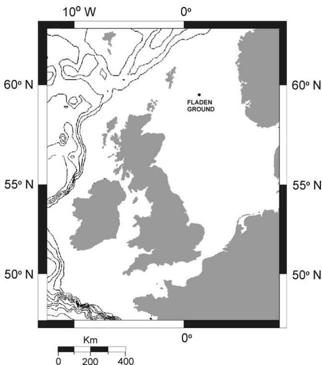
Figure 1 Location of A. islandica specimens collected from the Fladen Ground, northern North Sea. The valves used to construct the chronology were dead-collected in a single trawl by the RV Scotia in 2001 (s01 trawl 197) in 115 m water depth at 58°49.86'N, 0°21.35'W
