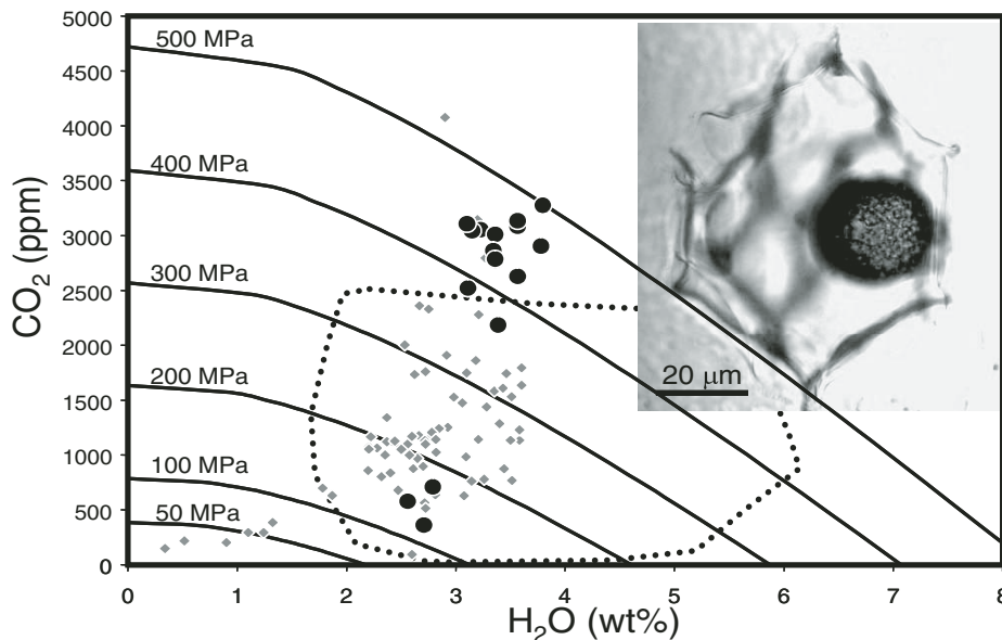
Figure 3. Relationships between H 2 O and CO 2 contents in melt inclusions from fall-stratified (FS) olivine (circles), phenocrysts in recent Mount Etna lavas (diamonds; after Métrich et al., 2004; Spilliaert et al., 2006), and arc basalts (dotted outline; after Wallace, 2005). Note that adequate comparison of data from different sources requires normalization to same degree of fractionation. Isobars are calculated at 1220 °C and 47.5 wt% SiO 2 in melt using Volatilecalc (Newman and Lowenstern, 2002). Inset shows typical H 2 O- and CO 2 -rich silicate melt inclusion with CO 2 -vapor bubble in FS olivine. Bubble walls are coated by tiny Ca-Mg-bearing carbonates (determined by laser Raman spectroscopy, GeoForschungsZentrum Potsdam, Germany), thus initial CO 2 content was even higher than measured.
