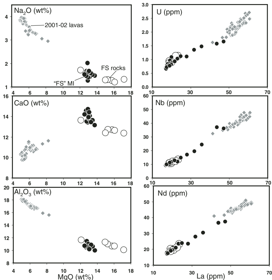
Figure 2. Comparison between compositions of fall-stratified (FS) parental magmas (exemplified by recalculated melt inclusions), FS whole rocks, and modern lavas of Mount Etna (Andronico et al., 2005; Corsaro et al., 2006). Note significant variations in trace elements among individual melt inclusions. Symbols as in Figure 1.
