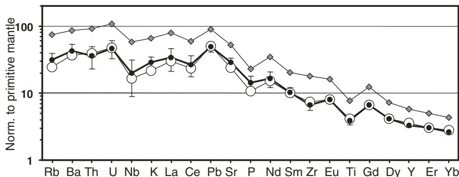
Figure 1. Primitive mantle normalized (after Sun and McDonough, 1989) trace element compositions of fall-stratified (FS) rocks (open circles, average of 6 samples), melt inclusions hosted in FS olivine phenocrysts (closed circles, average of 23 melt inclusions; bars show one standard deviation), and Mount Etna lavas erupted in 2001–2002 (diamonds, average of 61 samples; after Andronico et al., 2005; Corsaro et al., 2006).
