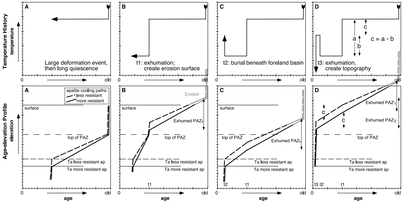
Figure 5. Schematic illustration of the effect of differing total annealing temperatures ( T_a ) on complex cooling paths. The four vertical elevation profiles represent a sequence of exhumation (cooling) and burial (reheating) events. (top) Evolving temperature history and (bottom) distribution of apatite fission track ages in a vertical profile at the corresponding time step. Each profile shows the cooling path of apatites that are more (solid line) and less (dashed line) resistant to annealing. The base of the partial annealing zone (PAZ) for each type of apatite is considered to be the respective T_a . Exhumation and burial events are (unrealistically) depicted as instantaneous for clarity. The geothermal gradient is assumed to remain constant and advection of isotherms is neglected for simplicity. (a) A large deformation event followed by a long period of quiescence gives shallow samples a common age. More resistant apatites are reset at lower elevation (hotter temperature); therefore the slope of the more resistant cooling path is steeper in the PAZ. (b) Large exhumation event at time t_1 forms exhumed PAZ 1 . A new PAZ forms at depth. (c) Section buried and reheated beneath sediments of a sedimentary basin at time t_2 . Heating resets all apatites below their respective T_a . Exhumed PAZ 1 is partially reset. In the lower part of the current PAZ, cooling paths for apatites with different T_a may be parallel. If the exhumation event was large enough to shift the entire PAZ 1 to a temperature hotter than the appropriate T_a , then the exhumed PAZ 1 would be completely overprinted. (d) A second large exhumation event that creates new exhumed PAZ 2 at time t_3 . Ongoing exhumation could subsequently expose the entire exhumed PAZ in mountainous topography. If the simplifying thermal assumptions are correct, the shape of the age-elevation curve can be used to reconstruct the magnitude of thermal events. The difference between the magnitude of exhumation t_1 (Figure 5a) and burial (Figure 5b) is equal to the difference between the base of PAZ 1 and the base of PAZ 2 (Figure 5c) (for a given apatite type). Therefore, if the base of PAZ 1 and PAZ 2 can be determined and the magnitude of burial can be constrained by thermal modeling or independent geological data, it is possible to estimate the magnitude of exhumation that occurred at t_1 .
