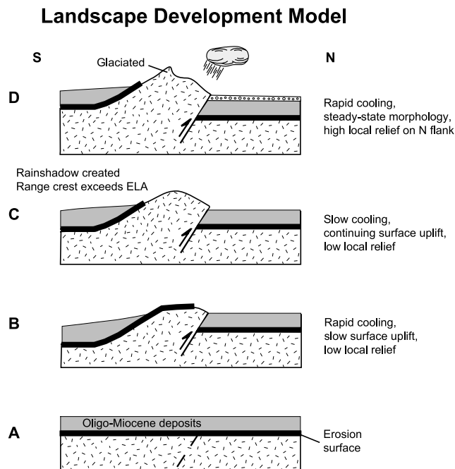
Figure 8. Schematic evolution of topography in the Kyrgyz range, showing the effect of contrasting lithologies on exhumation and surface uplift rates. (a) Oligocene–early Miocene foreland basin deposited above regional erosion surface. (b) Rapid exhumation of sediments in hanging wall of thrust causing rapid cooling but slow surface uplift of range. (c) Area of exposed basement increasing relative to young sedimentary cover, and erosion rates decreasing, leading to increasing surface uplift rates. (d) Range becoming large enough to create a significant orographic barrier; subsequently placing upper portion of range above equilibrium line altitude (ELA). Glacial erosion causes drainage basins on windward side to expand at the expense of more arid, less deeply incised basins on the leeward side.
