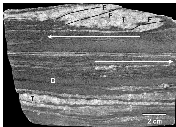
Figure 5. Polished hand sample of mylonitic Pierre's Pond suite diorite and tonalite from Star Lake, illustrating highly strained character of the diorite (D) and tonalite (T). Note folding (F) and stretching (arrows) of tonalite veins within the foliation planes.
