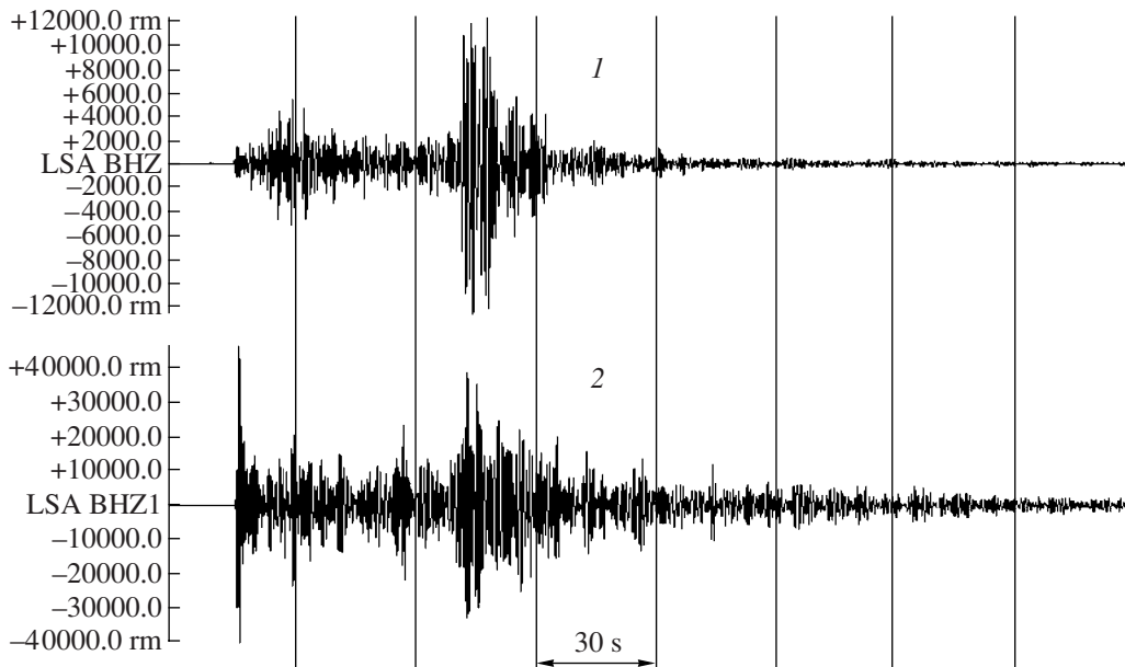
Fig. 2. Examples of seismograms obtained at LSA station (vertical component, filter 1.25 Hz). (1) August 5, 2000; 31.85^\circ \text{ N} , 94.43^\circ \text{ E} ; h = 33 \text{ km} (north of the source zone); (2) November 30, 2002; 28.62^\circ \text{ N} , 95.07^\circ \text{ E} ; h = 31 \text{ km} (central part of the source zone).
