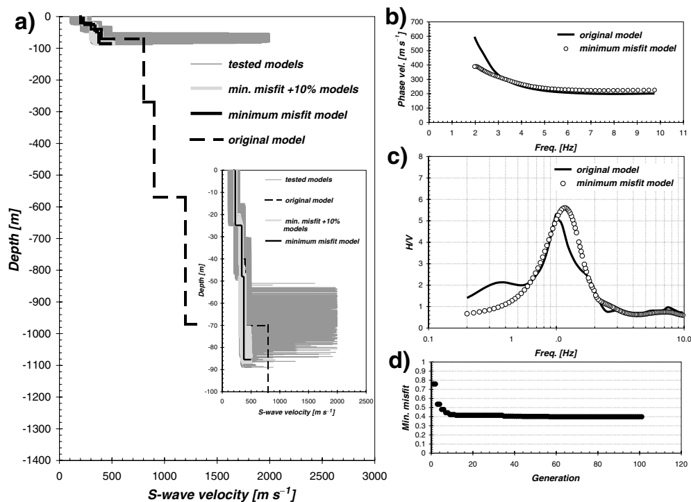
Figure A2. Joint inversion with GA. (a) S -wave velocity models. Inner inset: view of results at enlarged scale. (b) Rayleigh wave dispersion curves. (c) H/V spectral ratio curves. (d) Minimum misfit value (cost function eq. 1) as a function of generation.
