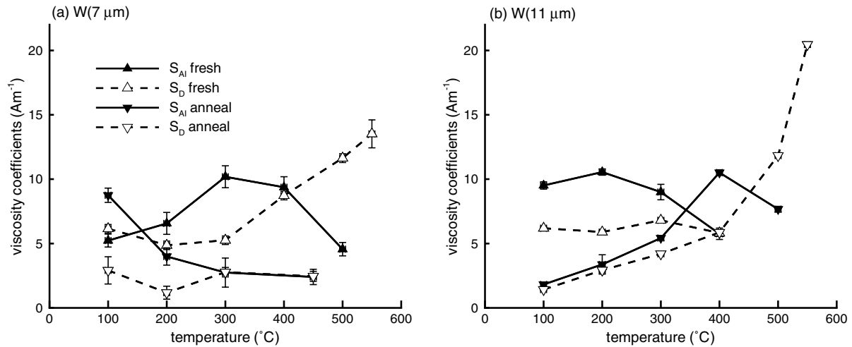
Figure 3. S_{\text{AI}} and S_{\text{D}} versus temperature for samples W(7 \mu\text{m}) and W(11 \mu\text{m}) for VM data before and after annealing. The samples were AF demagnetized at room temperature between each acquisition and decay measurement. The inducing field was 550 \mu\text{T} .
