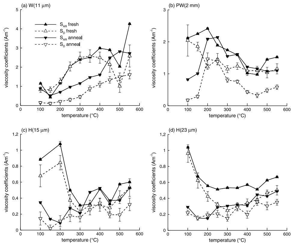
Figure 4. S_{\text{AR}} and S_{\text{D}} versus temperature for samples W(11 \mu\text{m}) , PW(2 \text{ mm}) , H(15 \mu\text{m}) , and H(23 \mu\text{m}) for VRM data before and after annealing. The samples were initially AF demagnetized, and then the viscosity was measured accumulatively. The inducing field was 2 \text{ mT} ( 2000 \mu\text{T} ).
