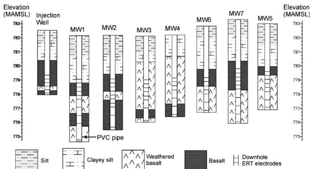
Fig. 2 Well logs for monitoring wells and the injection well (modified from Nimmer and Osiensky 2002a). Electrode locations are also shown
