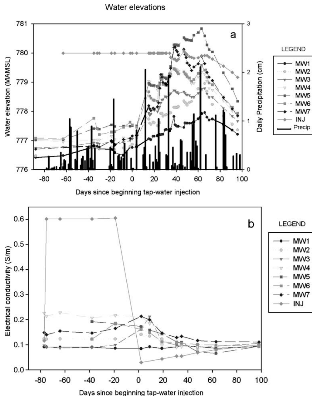
Fig. 4 a Graph of water-elevation measurements in the wells and precipitation in water equivalents. b Graph of electrical conductivity measurements of water in the wells. Day 0 represents the beginning of the tap-water injection
