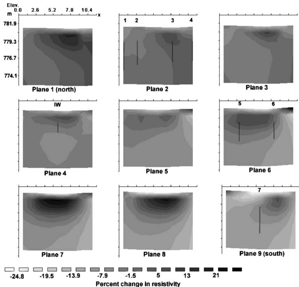
Fig. 7 Surface ERT resistivity distributions for t=68/t=17 d (land surface is at an elevation of 783.2 MAMSL): cross-sectional images. The thickness of each plane is 1.3 m. Lines on cross sections represent depths of electrode sections, and the numbers correspond to the well number (i.e., MW1 is represented by 1). When wells are located along the border of two cross-sections, the electrode lines are located on the northernmost cross-section. See Fig. 1 for well descriptions
