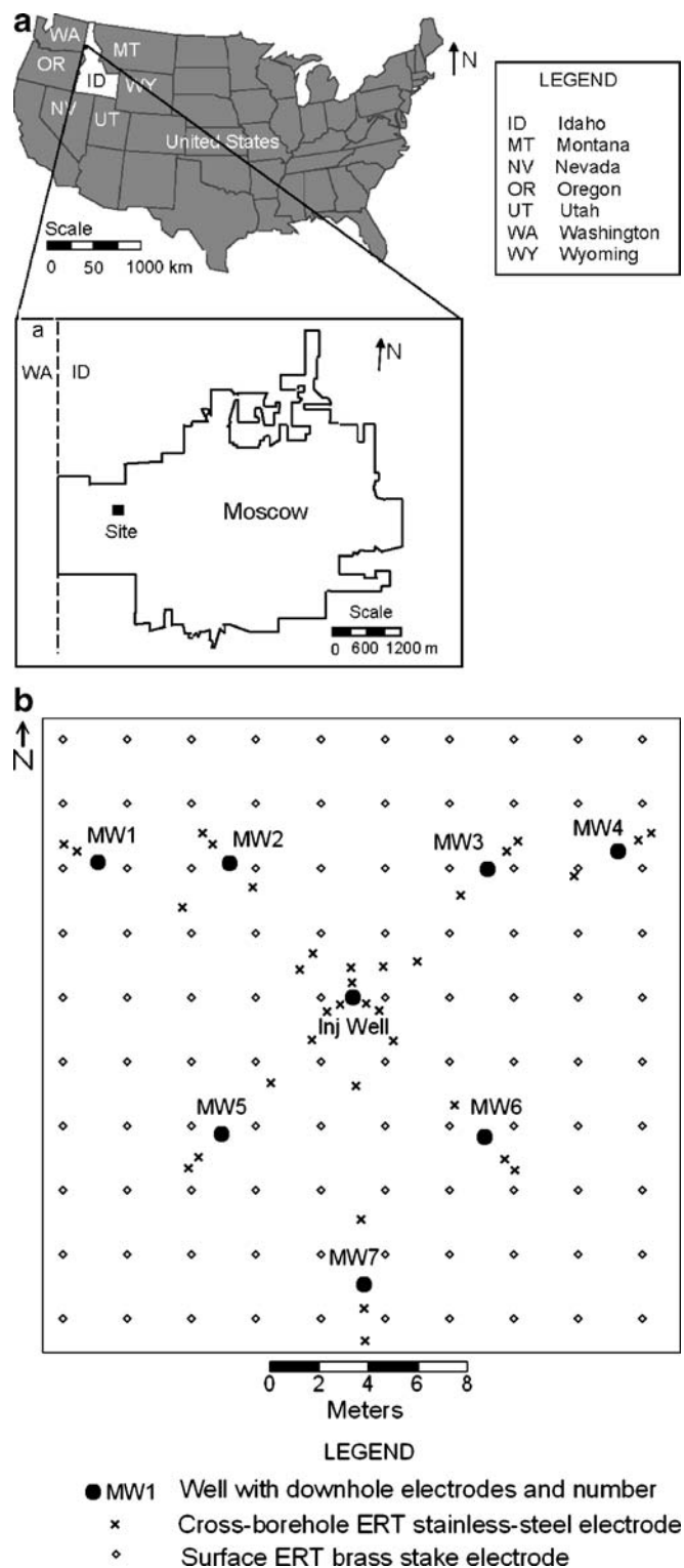
Fig. 1 a Map showing Idaho, USA and the study site at Moscow. b Location of wells and surface electrodes at the study site
