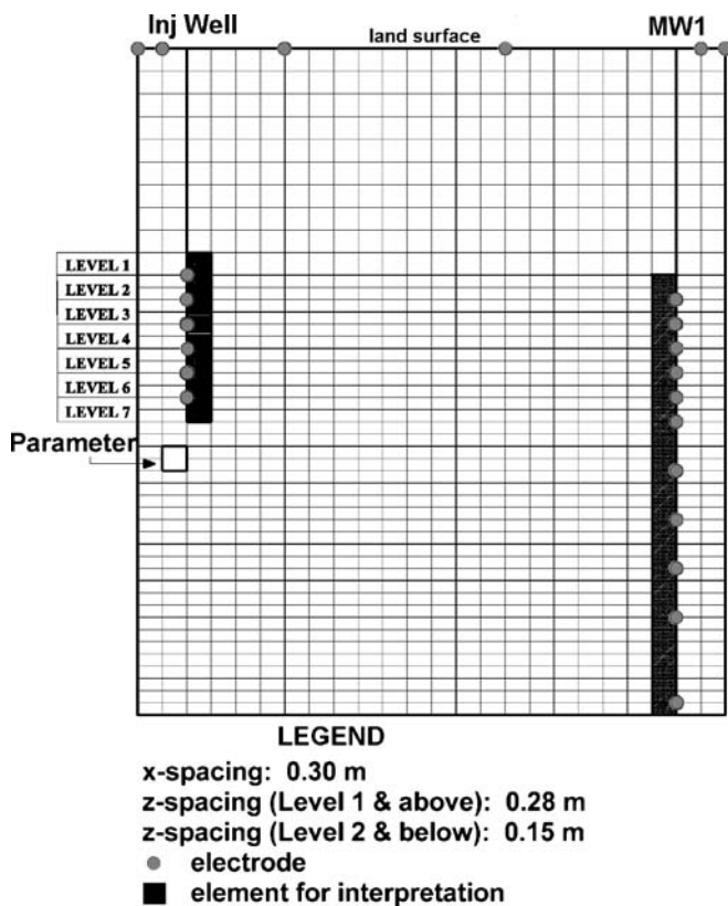
Fig. 3 Example cross-sectional subgrid for I-MW1
