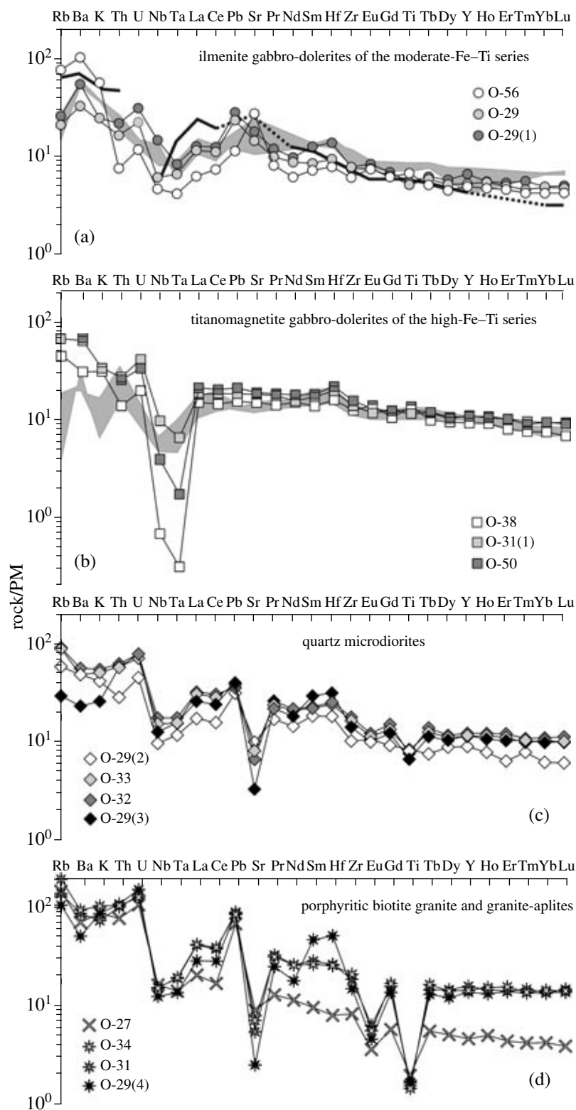
Fig. 9. Multielement patterns of the Lower Paleocene hypabyssal rocks of the Omgon Range. For comparison, the diagrams demonstrate similar patterns typical of the Upper Cretaceous–Middle Eocene volcanic rocks in extension zones in the continental margin of Northeast Asia (gray shading) (Fedorov and Filatova, 1999): (a) Hy -normative moderate-Ti tholeiitic basalts of Danian–Paleocene age from the Kakanaut area, (b) Hy -normative high-Ti tholeiitic basalts of Maestrichtian–Middle Eocene age from the Rarytkin area. The concentrations of elements are normalized to the primitive mantle (Hofmann, 1988).
