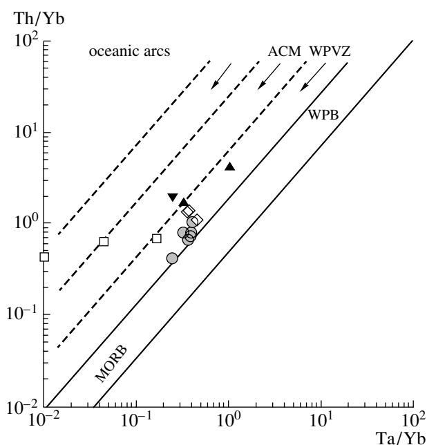
Fig. 7. Th/Yb–Ta/Yb diagram (Gorton and Schandl, 2000) demonstrating different ratios of highly incompatible elements in the hypabyssal rocks of the Omgon Range, the uncertain nature of the ilmenite gabbro-dolerites, and the similarity of the titanomagnetite gabbro-dolerites, quartz microdiorites, biotite granite, and granite-aplites to magmatic products at continental margins.
