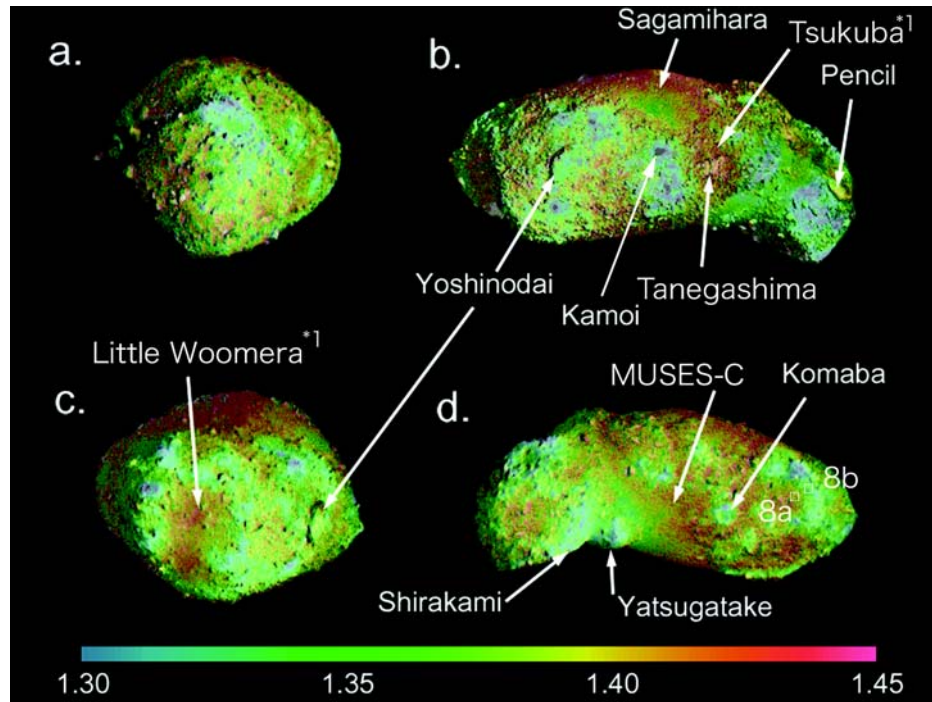
Fig. 2. False-color images of each hemisphere. Intensity is modulated by an underlying w-band image, and R_w/R_b ratio is shown in false color as hue (ST_2385559680-ST_2385598109, ST_2406717897-ST2406737168, ST_2407409109-ST2407428397, ST_2418659460-ST2418768895). The two boxes called “8a” and “8b” are the corresponding areas in Fig. 8.
