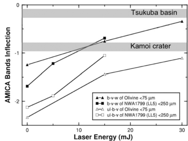
Fig. 5. Correlation between the amounts of ul-b-v-w inflections and the degree of space weathering (indicated by laser energy). C_v (b-v-w inflection) values of Tsukuba basin and Kamoi crater are also shown.
