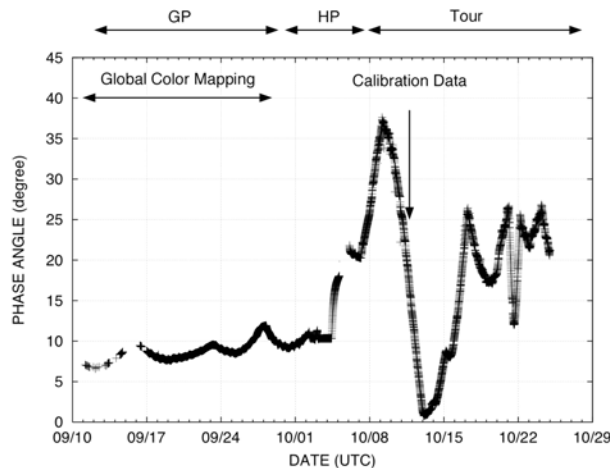
Fig. 1. Phase angle of AMICA boresight. The color data presented in this paper were obtained in the first three weeks at a phase angle of about 10^\circ , while a calibration factor was determined using the data collected on October 11, 2005, at a phase angle of 21^\circ .
