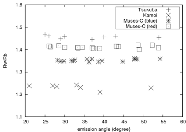
Fig. 3. Emission angle dependences of color ratio ( R_w/R_b ) in Kamoi crater (bluest crater), Tsukuba basin (one of the reddest regions), and the bluer (Yatsugatake side) and redder parts (in the seashore) of MUSES-C Regio.
