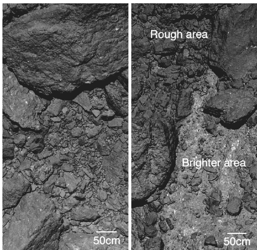
Fig. 8. Close-up images on the western side. Original lossless data were processed with the Lucy-Richardson image deconvolution algorithm in order to restore the blurred images. The spatial resolutions are 6 mm/pixel (left) and 9 mm/pixel (right). The left image (ST_2544579522) is of a ubiquitously rough area. The right image (ST_2544617921) is the boundary between a rough (boulder-rich) area and a brighter (fresher) area on the rim of LINEAR crater.
