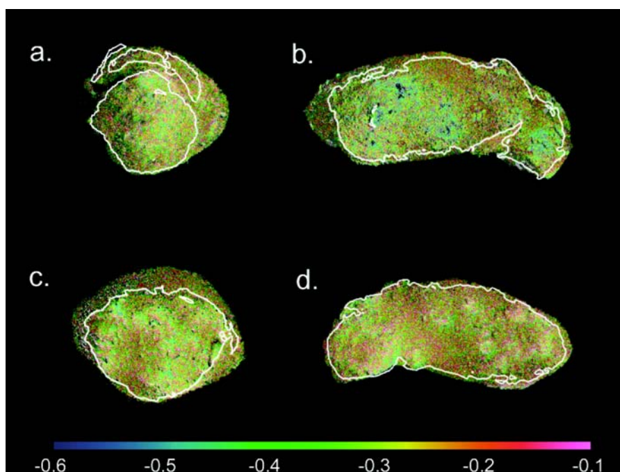
Fig. 7. Space-weathering index ( C_w , b-v-w inflection) map overlaying a w-band image. The solid line denotes the boundary of the incident angle of 60^\circ ; at less than this angle, the index accurately shows the degree of space weathering.
