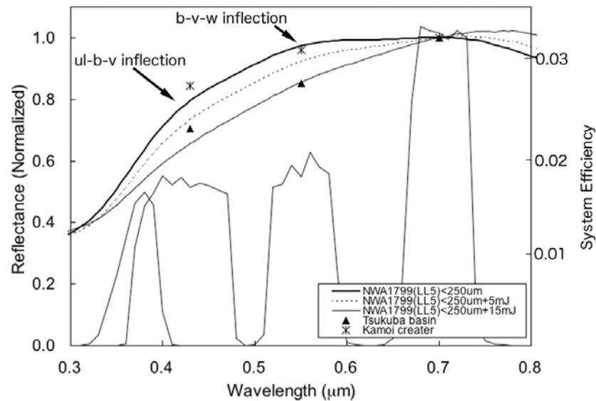
Fig. 4. Plots of visible reflectance spectra of fresh and laser-irradiated LL5 chondrite samples. Example reflectance in Tsukuba basin and Kamoi crater are also plotted. The system efficiencies, which are the predicted throughput performance of the AMICA optical system and CCD quantum efficiency, are drawn for reference.
