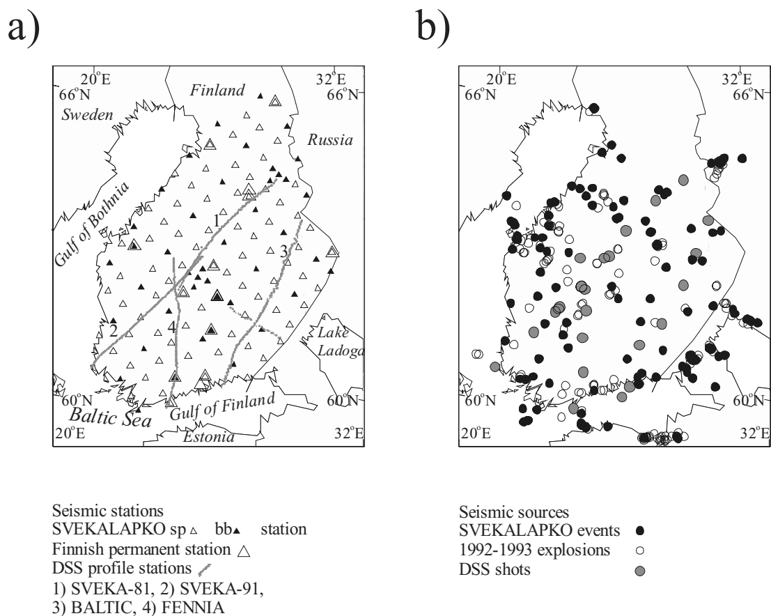
Figure 2. Seismic stations (a) and sources (b) used in this study. The maps are plotted using the Generic Mapping Tool—routines (Wessel & Smith 1998).
