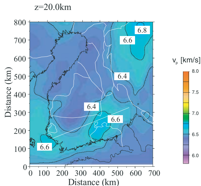
Figure 9. P -wave velocity model at depth of 20 km plotted from the velocity matrix of Sandoval et al. (2003) model (courtesy of Senen Sandoval). Corresponding depth slice of our model is shown in Fig. 6(a), z = 20 km.
