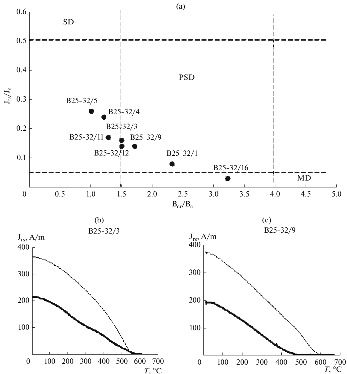
Fig. 7. A Day diagram (a) and curves of thermomagnetic analysis J_{rs}(T) for samples where the main carrier of magnetization is magnetite (b) and titanomaghemite (c).
