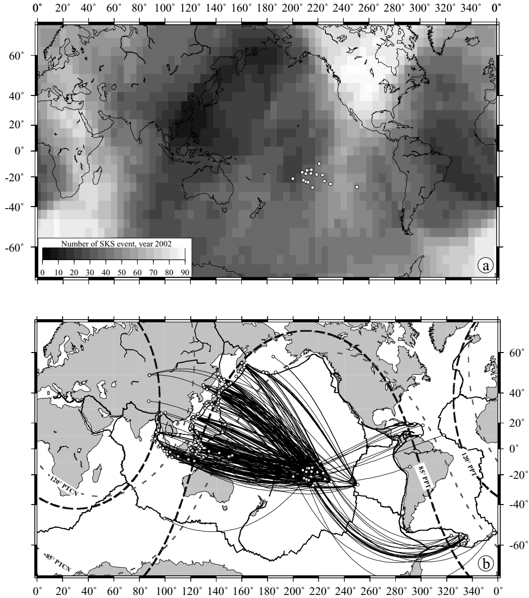
Figure 2. (a) Global map showing the density of recordable events ( m_b > 6.0 ) occurring at epicentral distances in the range 85\text{--}120^\circ for the year 2002. White/dark colours represent areas with a large/small number of observable SKS events. French Polynesia lies in a rather unfavourable situation with about 30 potentially usable events per year. (b) Location of the events that contributed to the 300 splitting measurements of this study, 60 of which being ‘non-null’ events. Great circles represent the 85^\circ and 120^\circ epicentral distances from stations PPT (thick dashed lines) and PTCN (thin dashed lines) to better visualize the location of the seismic sources that can potentially be used for SKS splitting studies in the South Pacific area.
