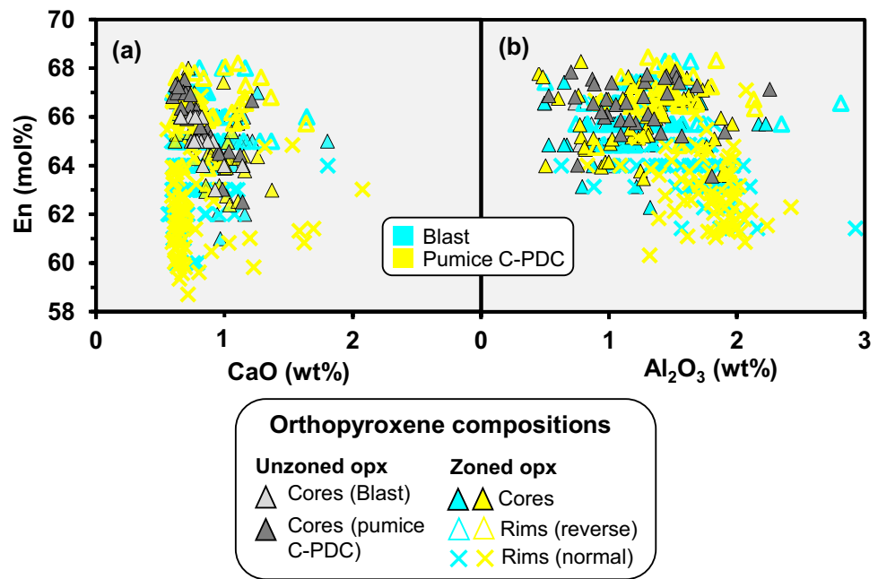
Fig. 8 Orthopyroxene compositions illustrated as the enstatite mol% versus a CaO wt% and b \text{Al}_2\text{O}_3 wt%, for unzoned phenocrysts (light grey triangles for blast samples and dark grey triangles for C-PDC pumices) and zoned phenocrysts showing compositions of cores and rims (for reverse and normal zonings); the blue and yellow symbols are for the blast samples and C-PDC pumices, respectively
