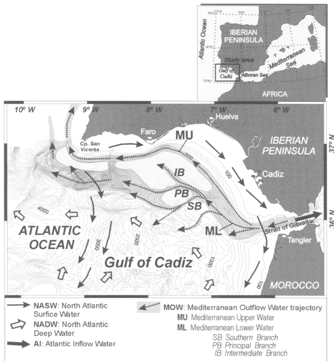
Fig. 1. Location of the Gulf of Cadiz in a regional bathymetric map (Heezen & Johnson 1969) indicating the general circulation patterns of MOW. (Modified from Hern  ndez-Molina et al. 2003.)
