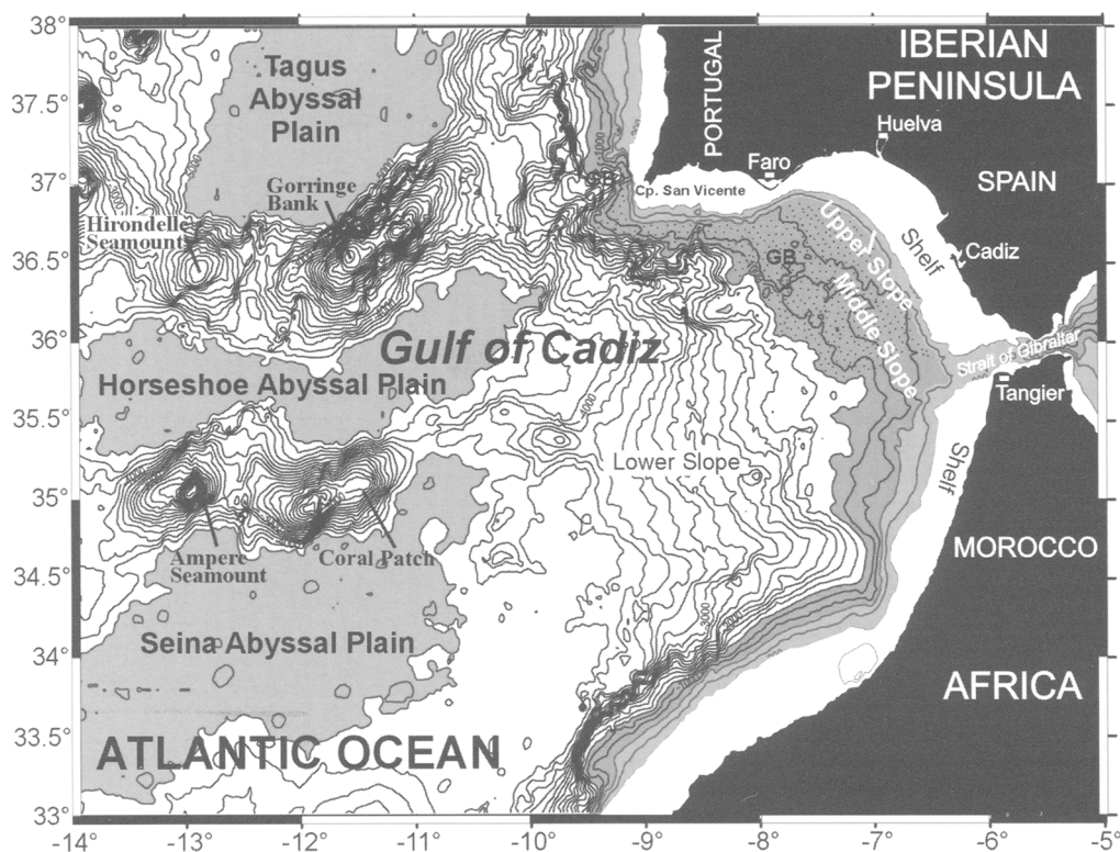
Fig. 2. Regional bathymetric map (in metres, from satellite data of Smith & Sandwell 1997) of the continental margin of the Gulf of Cadiz (modified from Hern  ndez-Molina et al. 2006). The contourite depositional system (CDS) of the Gulf of Cadiz is shown by the dotted area.
