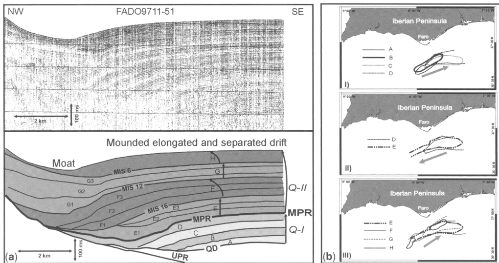
Fig. 12. (a) Sparker seismic profile and line drawing through the eastern zone of the Faro–Albufeira mound located in Sector 4, indicating the main seismic units within the Quaternary contourite sedimentary record. The change related to the MPR discontinuity should be noted. Also, a change from a sigmoid progradational configuration of the oldest sequences (A–G) to a more progradational stacking pattern of the two youngest sequences (G and H) can be identified (see Fig. 4 for location). (b) Sketches of the changes observed in the western zone of the Faro–Albufeira mound depositional sequences depocentres.
