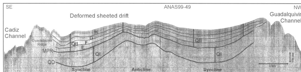
Fig. 15. Sparker seismic profile and line drawing through part of the deformed sheeted drift located in Sector 3 affected by low-frequency, low-amplitude anticline–syncline structures (see Fig. 4 for location).
