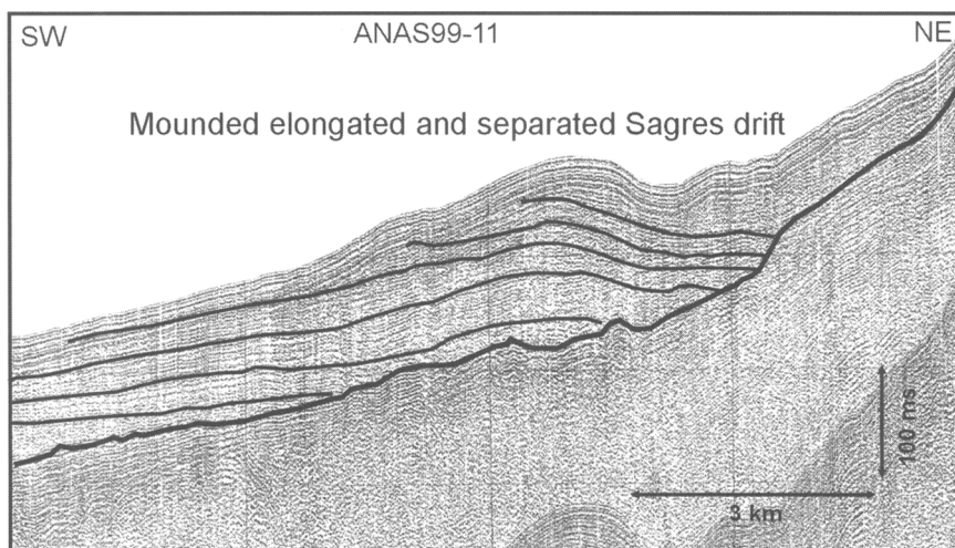
Fig. 13. Sparker seismic profile of the mound Sagres drift located in Sector 5, which displays a sigmoid to oblique–parallel configuration along a discontinuity at its base (see Fig. 4 for location).
