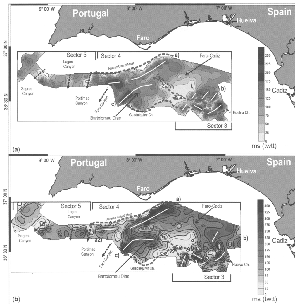
Fig. 7. Distribution and main depocentres of seismic units Q-I (a) and Q-II (b). The main depocentres are shown by white lines and lower-case letters.
