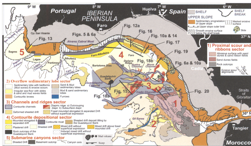
Fig. 4. Morphosedimentary map of the contourite depositional system on the middle slope of the Gulf of Cadiz with the location of the seismic examples (sparkler seismic profiles). Morphosedimentary sectors: (1) proximal scour and sand ribbons sector; (2) overflow sedimentary lobe sector; (3) channels and ridges sector; (4) contourite depositional sector; (5) submarine canyon sector. (Modified from Hern  ndez-Molina et al. 2003.)
