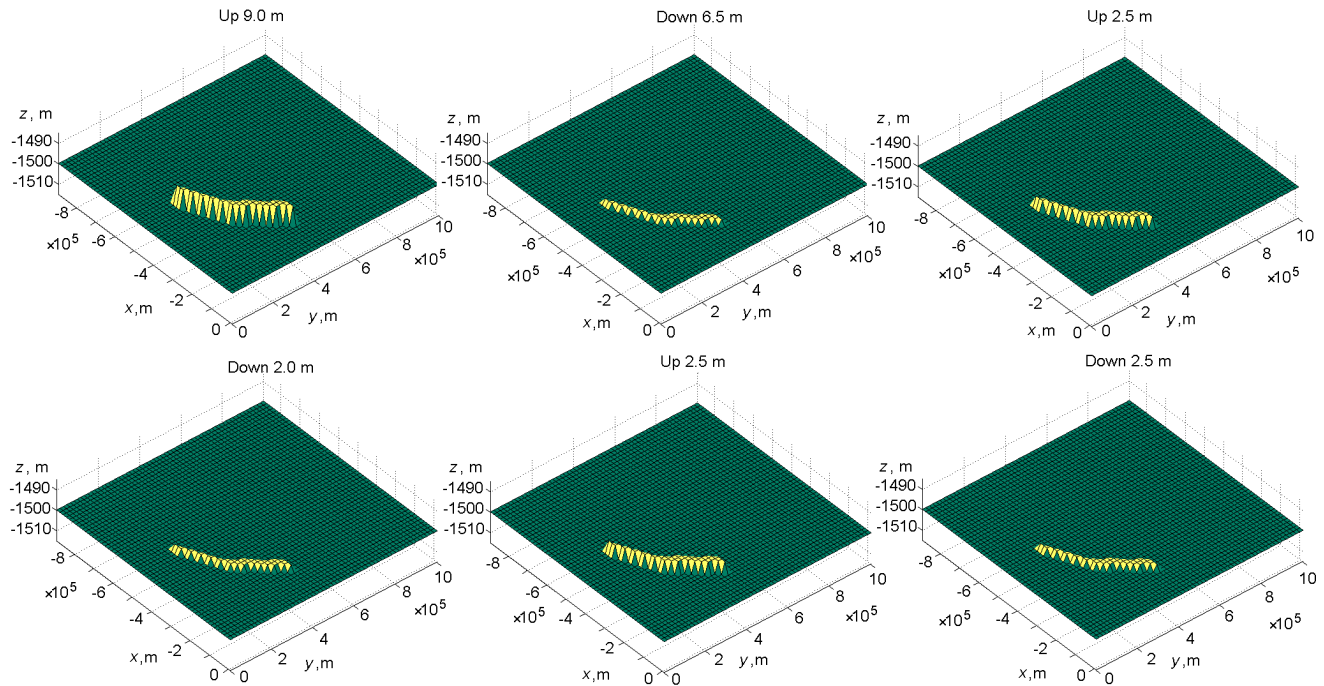
Figure 18. Illustration of dynamical model of seismic source with keyboard blocks. See also Animation 3 in online version.
