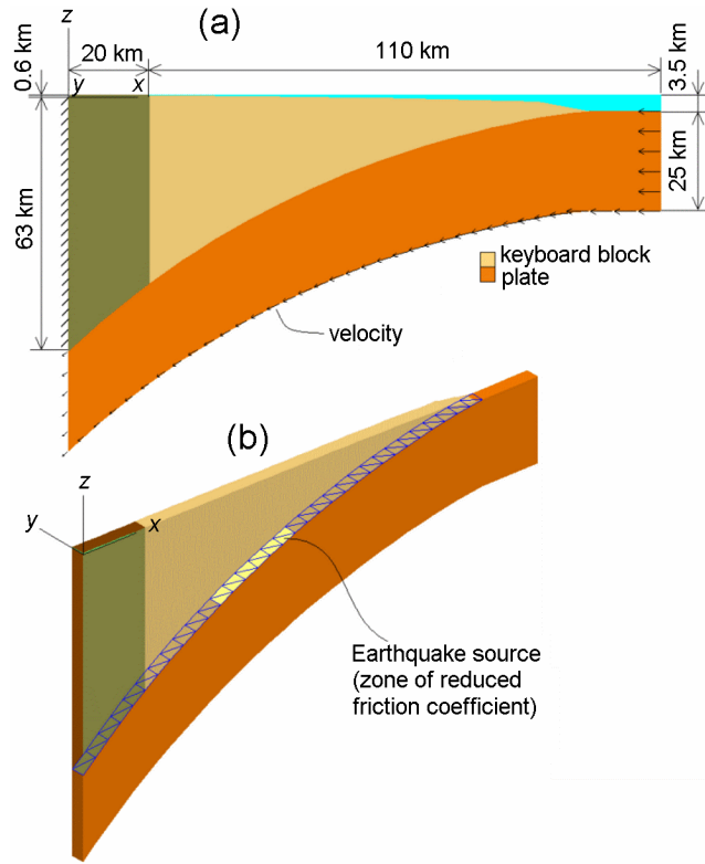
Figure 14. Sketch of the computational model subduction zone.
