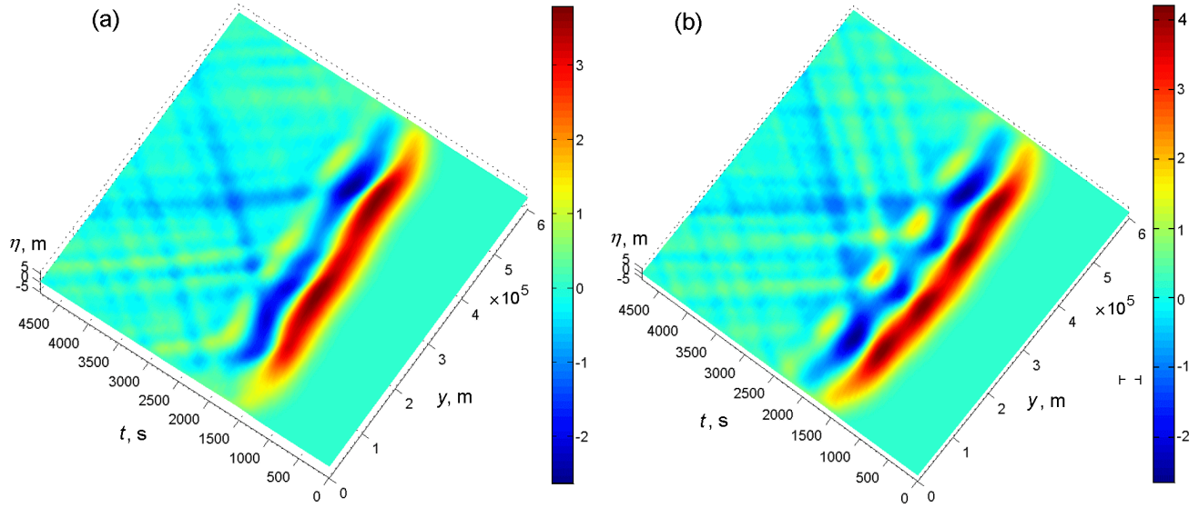
Figure 7. Space-time picture for the moving shoreline. y -axis is directed along the coast, height scale is in meters. (a) blocks of the same size, (b) blocks of different size.
