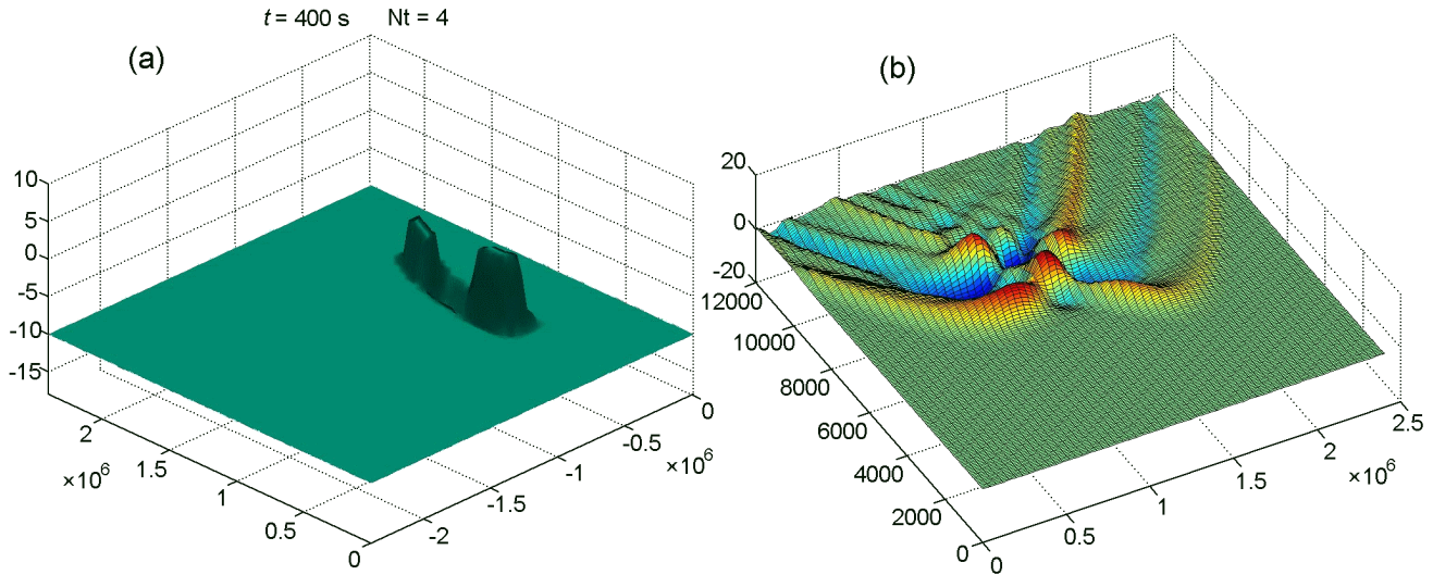
Figure 12. Modelling of the source of tsunamigenic earthquake 26 December 2004 by motion of three keyboard blocks rising along the subduction zone one after another from south to the north (a); space-time picture of the moving shoreline(b). Maximum run-up is equal to R_{\max} = 9.5 m, run-down R_{\min} = 7.5 m.
