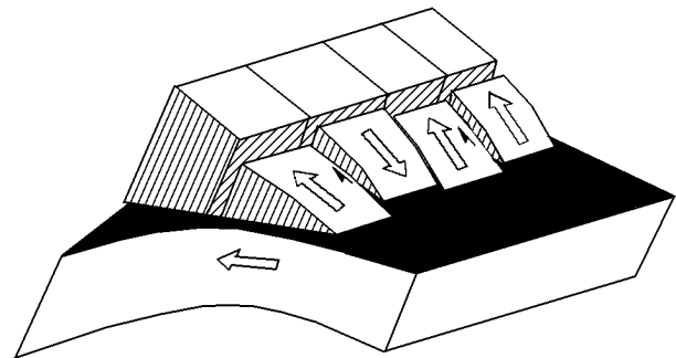
Figure 2. Keyboard model of the block structure in the frontal part of the island arc.
