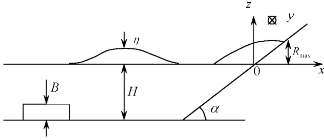
Figure 4. Geometry of generation and run-up of water wave at the sloping beach.
