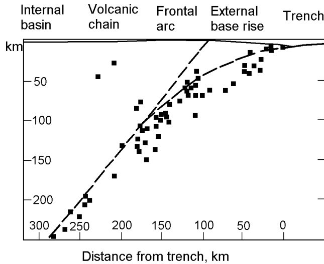
Figure 1. Sketch of subduction zone.
