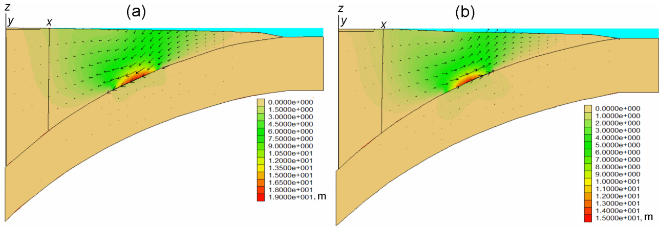
Figure 16. Distribution of residual displacements for the short (a) and long (b) time of elastic energy accumulation.
