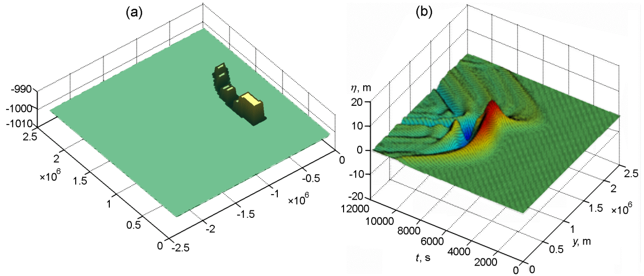
Figure 13. Modelling of the source of tsunamigenic earthquake 26 December, 2004 by motion of eight keyboard blocks moving along the subduction zone one after another from south to north (a); space-time picture of the moving shoreline(b). Maximum run-up is equal to R_{\max} = 11 m, run-down R_{\min} = 10 m.
