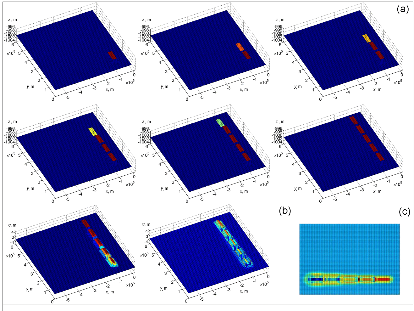
Figure 5. The example of successive block motion in earthquake source (a); The example of generation of surface water wave by seismic source: (b) for two time moments, (c) the view from upper point.
