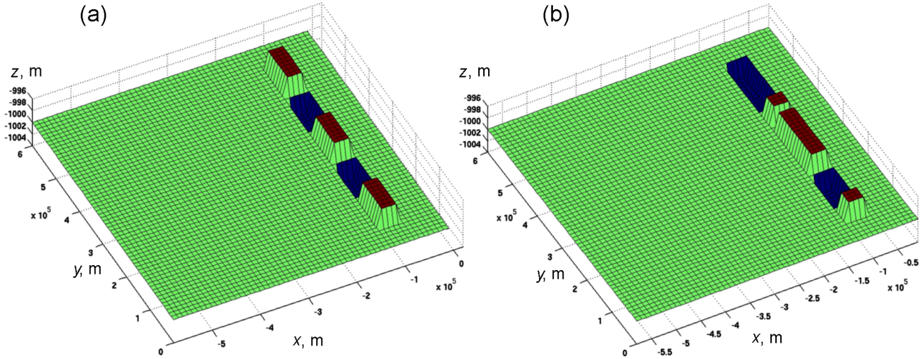
Figure 6. Successive motion of keyboard blocks in tsunamigenic earthquake source: the case of the same sizes blocks (a) and the case of blocks with different sizes (b).
