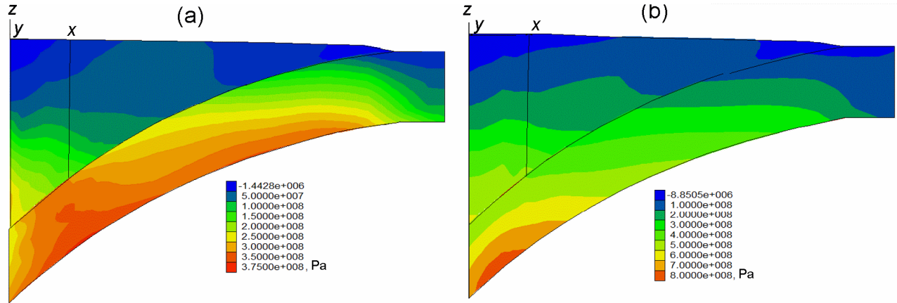
Figure 15. Distribution of the maximum shear stress for small (a) and large (b) time of elastic energy accumulation.
