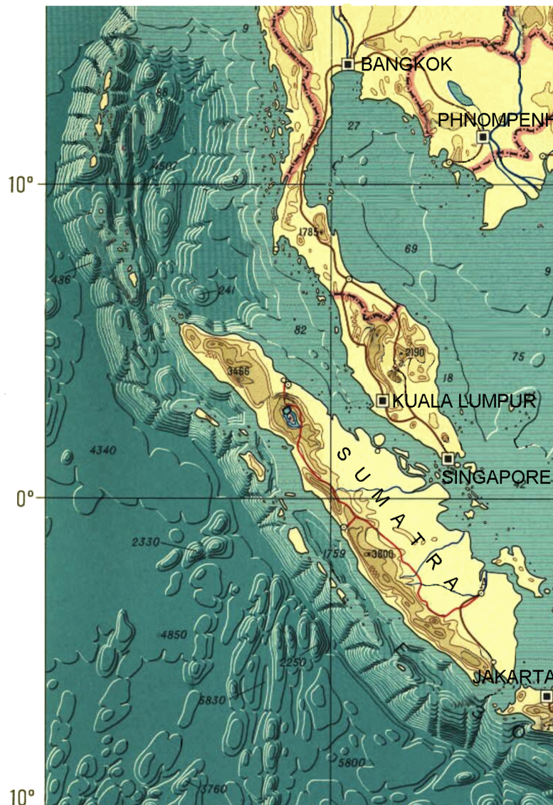
Figure 3. The bathymetric map of Philippine and Sunda arcs.
