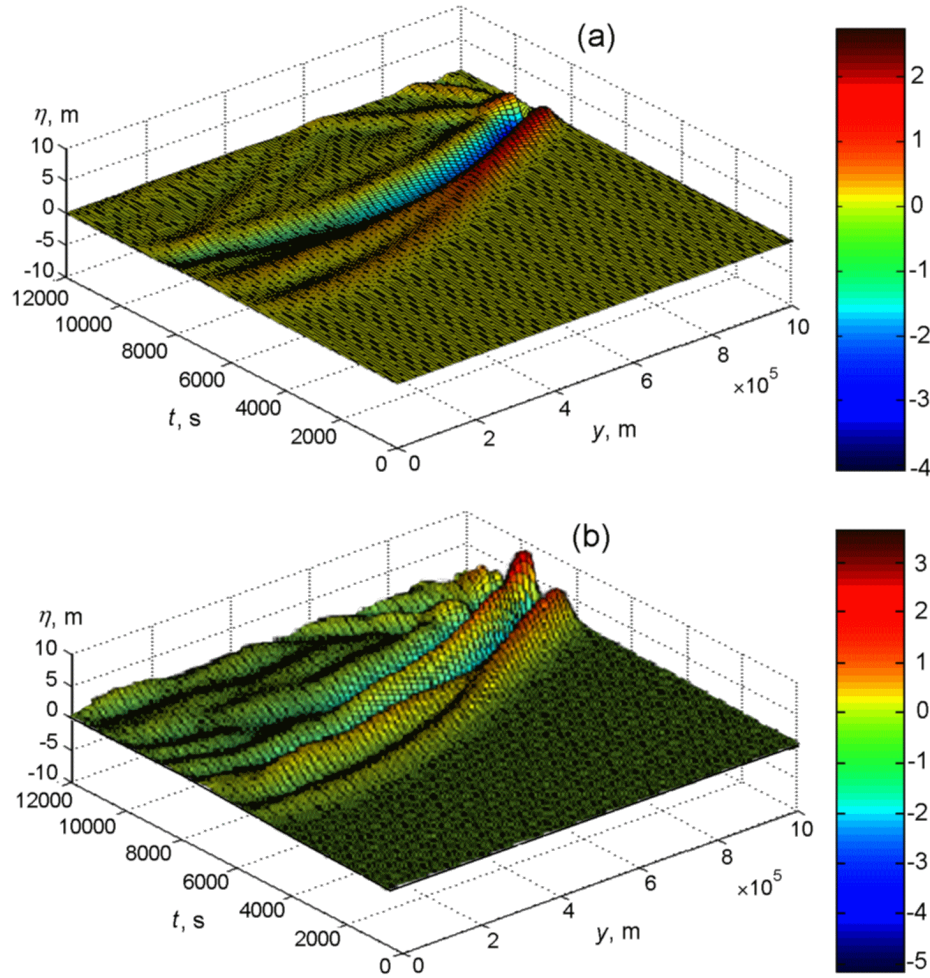
Figure 19. Space-time picture of wave distribution at the coming to a beach.
