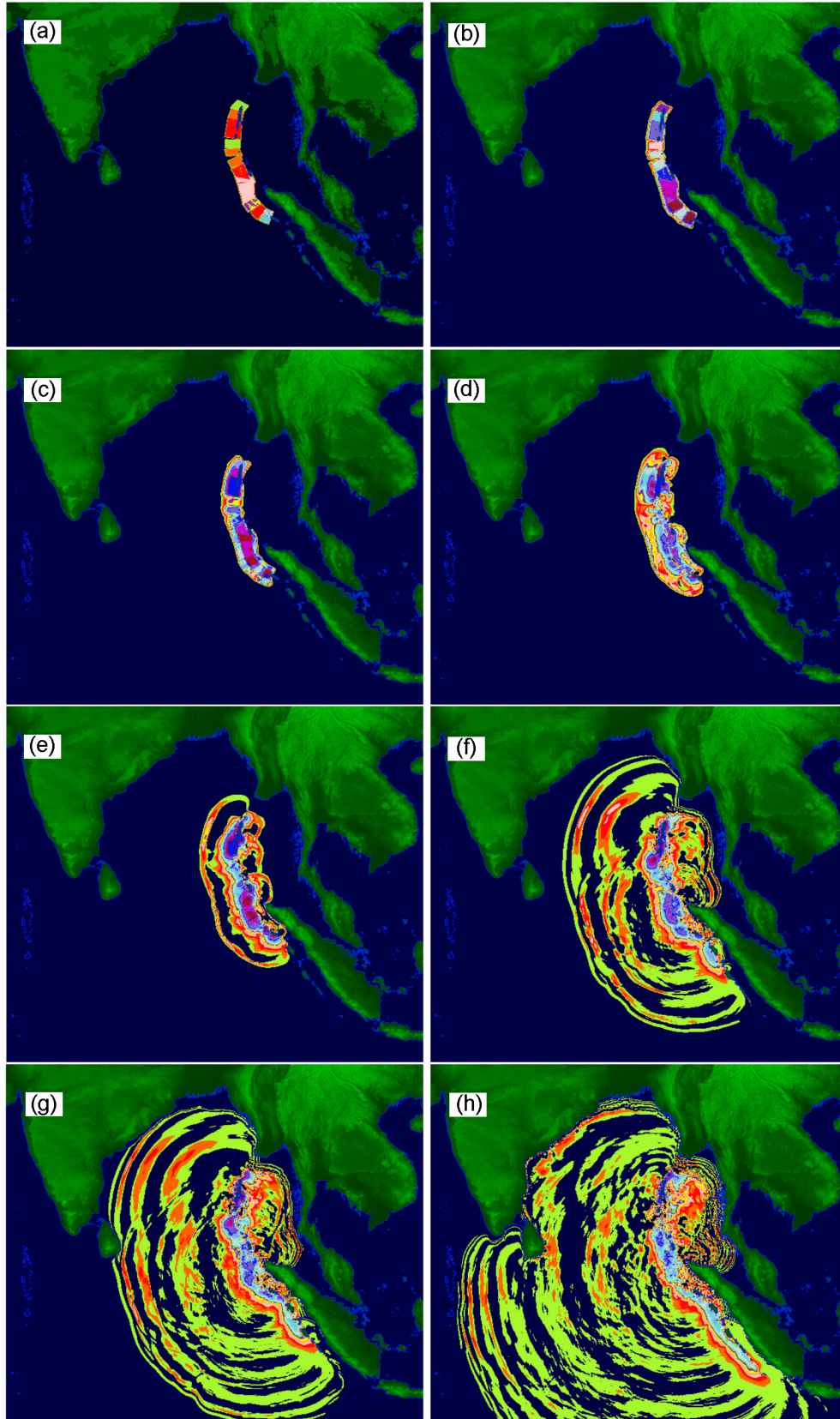
Figure 22. Generation and propagation of tsunami waves in the basin of the Indian Ocean for the seismic source comprising 14 blocks for the time moments: a – t=20'' , b – t=2'20'' , c – t=4'50'' , d – t=16'30'' , e – t=33'10'' , f – t=1h50' , g – t=2h30' , h – t=4h18' .
