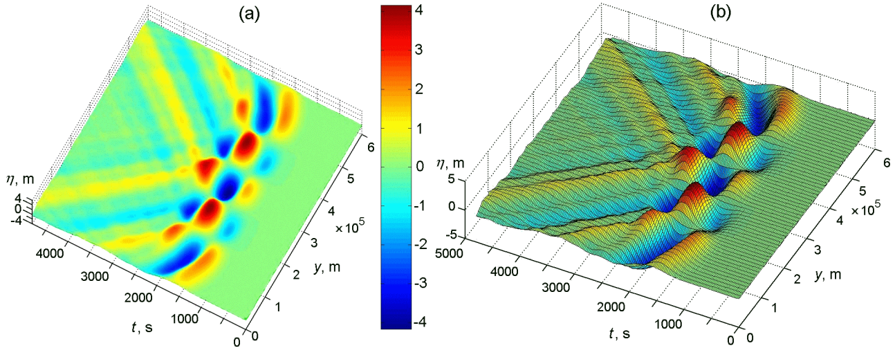
Figure 9. Space-time picture distribution of maximum wave run-up along shoreline for tsunami source consisting of keyboard blocks of the same size (Figure 6a); successive motion of blocks in the source: a) 2D simulation; b) 3D simulation.
