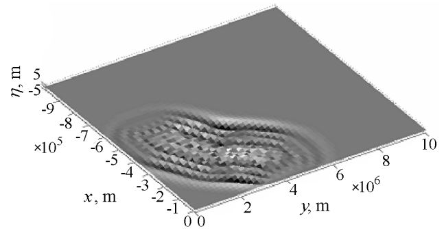
Figure 20. Generation of surface water wave by seismic source.
