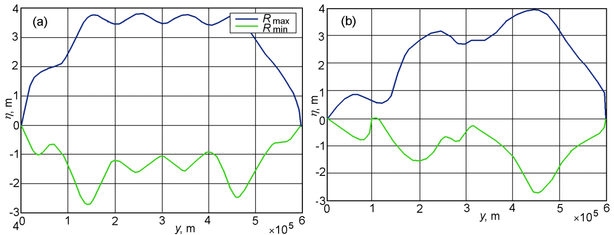
Figure 8. Distribution of maximum and minimum run-ups along 600 km part of the coast; y -axis is directed along the coast; R_{\max} is a maximum run-up; R_{\min} is a maximum run-down.
