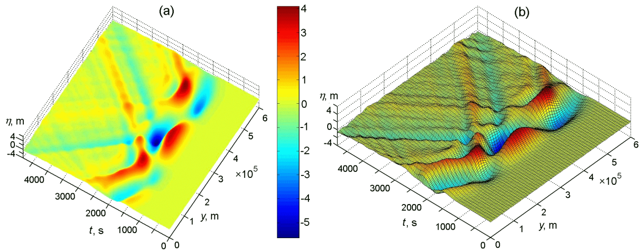
Figure 10. Space-time picture distribution of maximum wave run-up along shoreline for tsunami source consisting of keyboard blocks of the different size (Figure 6b); successive motion of blocks in the source: a) 2D simulation; b) 3D simulation.
