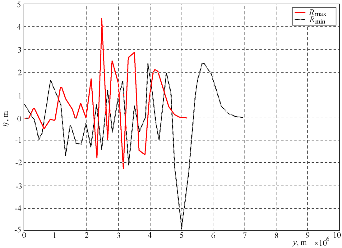
Figure 21. Distribution of values of run-up at the beach and run-down from the beach for moments of maximum run-up R_{\max} and run-down R_{\min} .
