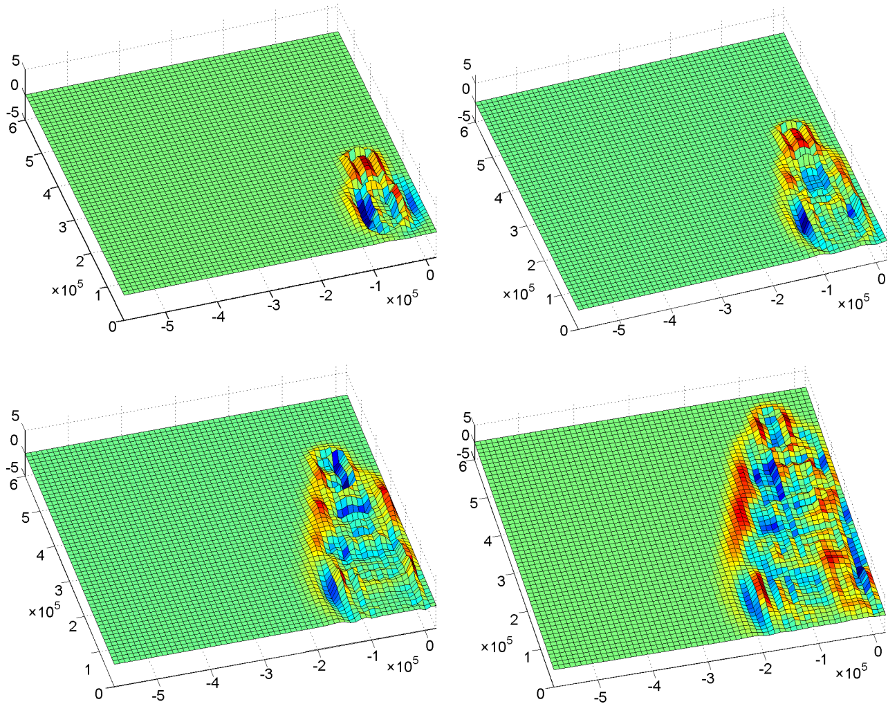
Figure 11. Propagation of surface water wave under rupturing in the source along the subduction zone.
