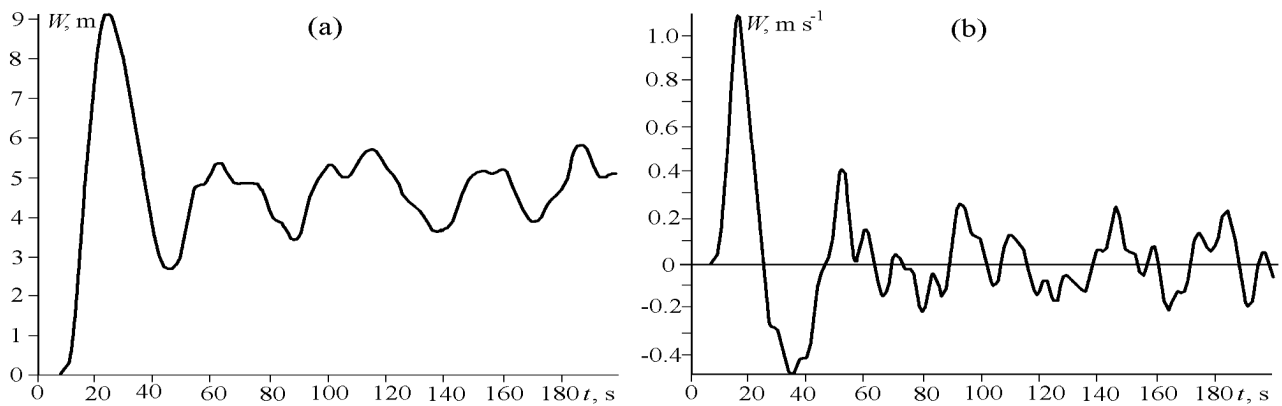
Figure 17. Time plots of vertical displacement (a) and vertical velocity (b) of sea bottom during the earthquake.
