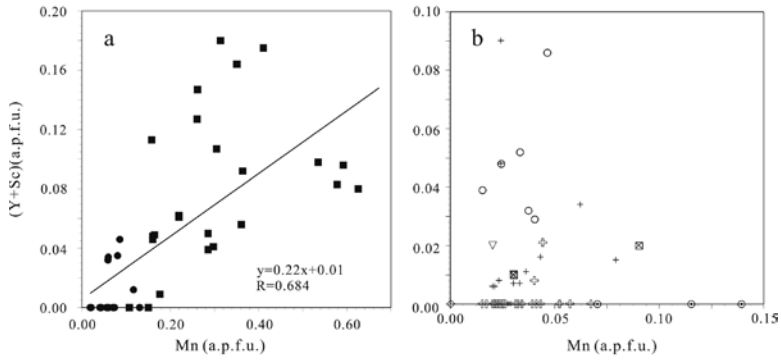
FIG. 6. Plot of (Y + Sc) versus Mn for (a) the allanite-(Ce) in our suite and (b) allanite-subgroup minerals from intracontinental settings and continental margins. Symbols are the same as in Figure 3.
