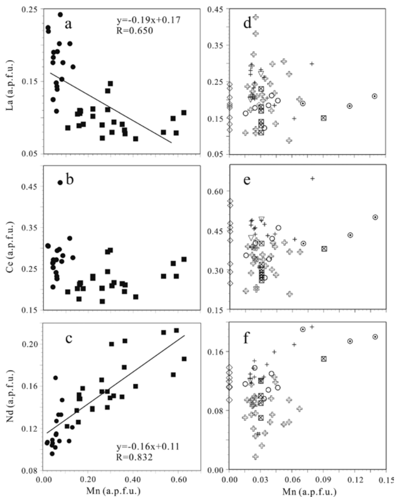
FIG. 5. Compositional variation between Mn and LREE (La, Ce, Nd) for (a–c) the allanite-(Ce) compositions in our suite and (d–f) allanite-subgroup minerals from intracontinental settings and continental margins. Symbols are the same as in Figure 3.
