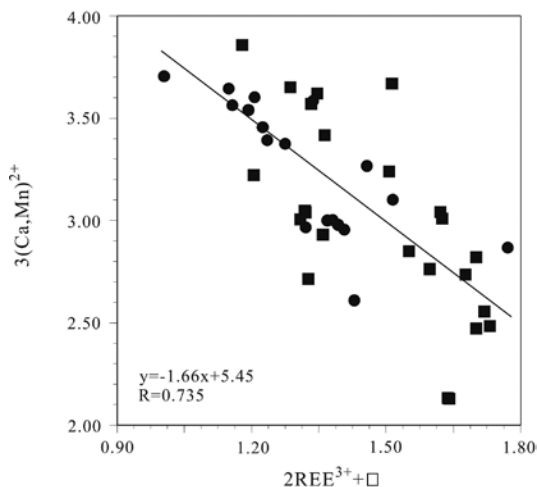
FIG. 4. Plot illustrating the potential coupled substitution at the A site of allanite-subgroup minerals from Japan. The substitution plotted is 3(\text{Ca,Mn})^{2+} \rightleftharpoons 2\text{REE}^{3+} + \square , where \square denotes a vacancy at the A site. Units: apfu ; symbols as in Figure 3.
