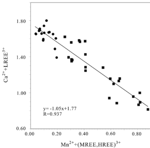
FIG. 8. Plots illustrating a potential coupled substitution between Mn-rich and Mn-poor allanite-(Ce) from granitic rocks, Japan. In all cases, LREE represents the total of La, Ce, Pr and Nd, and MREE = \Sigma(\text{Sm}, \text{Gd}, \text{Tb} and \text{Dy}) . HREE represents the sum of Y, Sc, Er, Tm and Yb. Symbols are the same as in Figure 3. Units: apfu .
