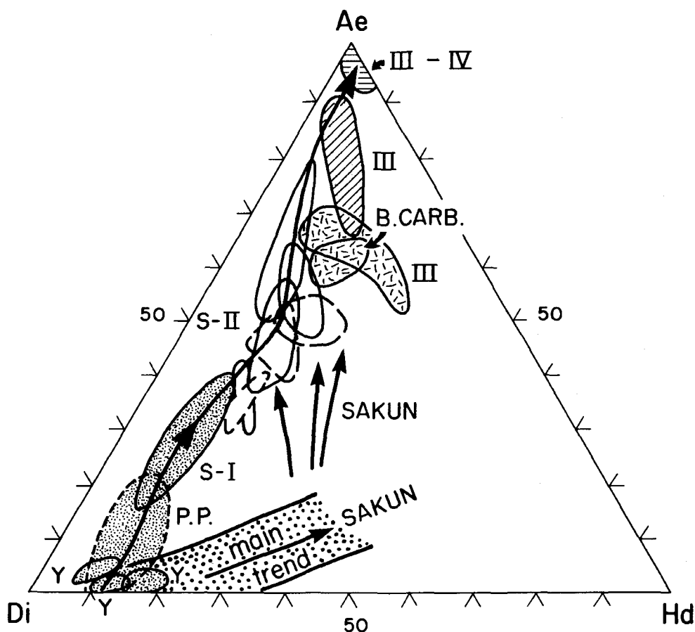
FIG. 11. Overall compositional trend (mol.%) of pyroxene occurring in Little Murun plutonic rocks depicted in the ternary system aegirine (Ae)- diopside (Di) - hedenbergite (Hd). Y = yakutite (kalsilitite pyroxenite); P.P. = phlogopite pyroxenite; S = shonkinite. B.CARB = benstonite carbonatite. Roman numerals indicate plutonic centres. Compositional trends for Sakun potassic complex (Aldan Shield) pyroxenes from Proshenkin and Sharygin (1990).
