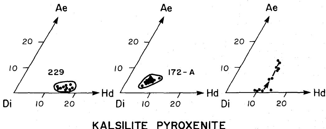
FIG. 2. Compositional variation of pyroxene in kalsilite pyroxenites.
