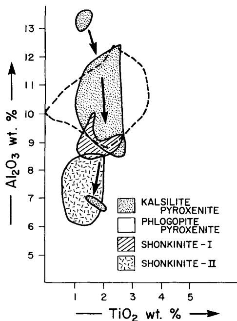
FIG. 9. Compositional fields, \text{Al}_2\text{O}_3 vs. \text{TiO}_2 , for mica occurring in Little Murun plutonic rocks.
