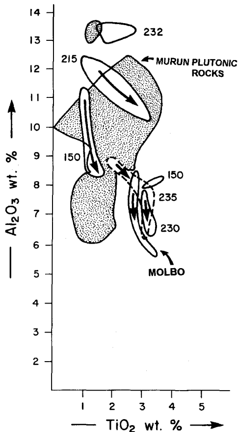
FIG. 10. Compositional fields, \text{Al}_2\text{O}_3 vs. \text{TiO}_2 , for mica occurring in 'lamproite-like' hypabyssal rocks.
