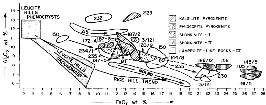
FIG. 8. Compositional variation, Al 2 O 3 vs. FeO T , for all Little Murun mica. Compositional trends for mica from Leucite Hills (Wyoming) and Rice Hill (Australia) lamproites from Mitchell and Bergman (1991).
