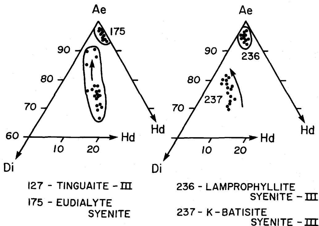
FIG. 6. Compositional variation of pyroxene in centre-III tinguaitite and late-stage mineralogically complex hypabyssal rocks.
