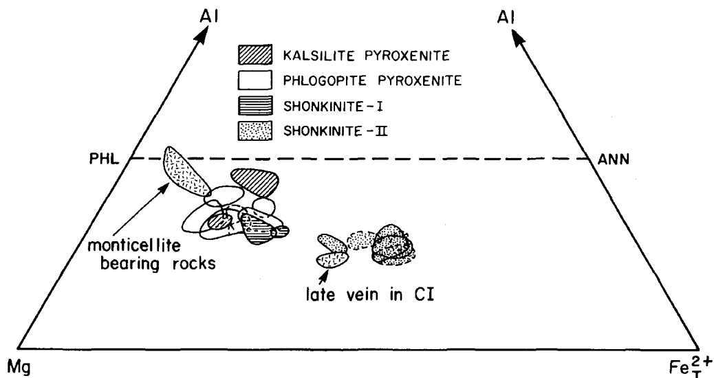
FIG. 7. Compositional variation of mica depicted in the ternary system Al-Mg-Fe T . PHL = phlogopite; ANN = annite.
