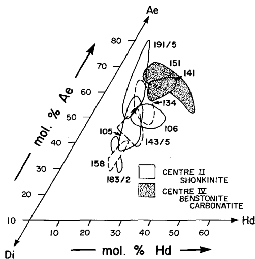
FIG. 5. Compositional variation of pyroxene in centre-II shonkinites and centre-IV benstonite carbonatites.
