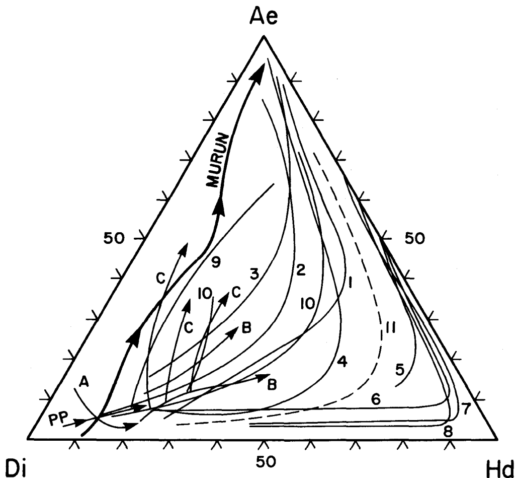
FIG. 12. Overall trend of pyroxene compositions (mol.%) in the Little Murun ultrapotassic complex compared with trends found in other alkaline rocks: 1 Morotu; 2 Uganda; 3 Itapirapua; 4 South Qoroq; 5 pantellerite; 6 Nandewar; 7 Ilimaussaq; 8 Coldwell centre-I; 9 Turja; 10 Iron Hill; 11 Coldwell-II; A,B,C, Fen. See Mitchell and Platt (1982) for data sources.
