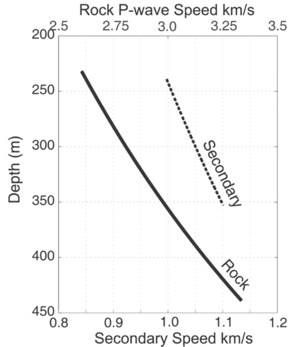
Fig. 10. A comparison of compressional P-wave and secondary wave velocities as determined using polynomial fitting.
