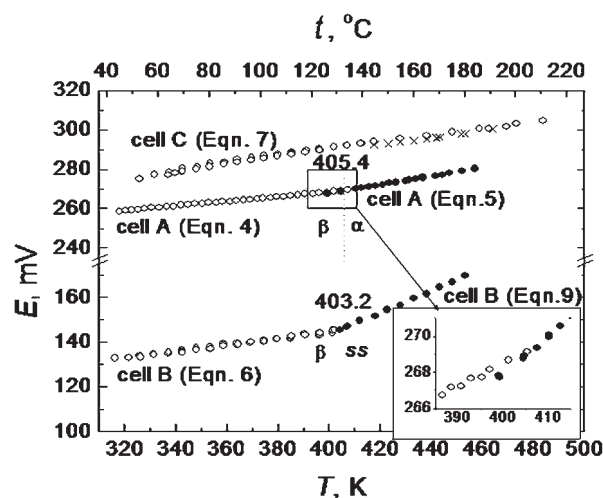
FIGURE 2. Temperature dependences of the EMF( E ) of Cells A, B, and C. The reproducible over-cooling of Cell A is shown in inset; b.c.c. denotes \text{Ag}_{2-x}\text{Au}_x\text{Se}_2 solid solution. Cross symbols show the reproducible hysteresis and mark the data points obtained under decreasing temperature regime (see Table 3, unaccounted points).
