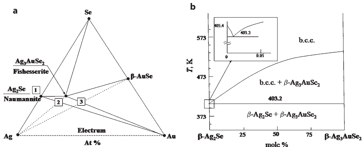
FIGURE 1. (a) Phase relations in the system Ag-Au-Se at 298–403 K and total Ar-gas pressure of 1 atm. The numbers of studied phase reactions 1, 2, and 3 are given in boxes. (b) Temperature-composition diagram for the pseudobinary system \text{Ag}_2\text{Se-Ag}_3\text{AuSe}_2 (after Wiegiers 1976). The eutectoid position is shown in inset; b.c.c. denotes solid solution with body-centered cubic lattice.
