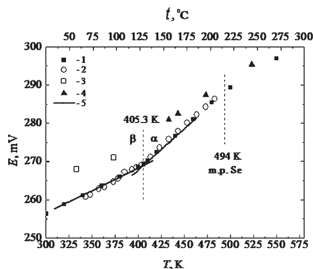
FIGURE 3. EMF ( E ) vs. temperature dependences for the reaction of naumannite formation from the elements according to different sources: 1 = Gronvold et al. (2003); 2 = von Oehsen and Shmalzried (1981); 3 = Takahashi and Yamamoto (1970); 4 = Kiukkola and Wagner (1957); 5 = this study.
