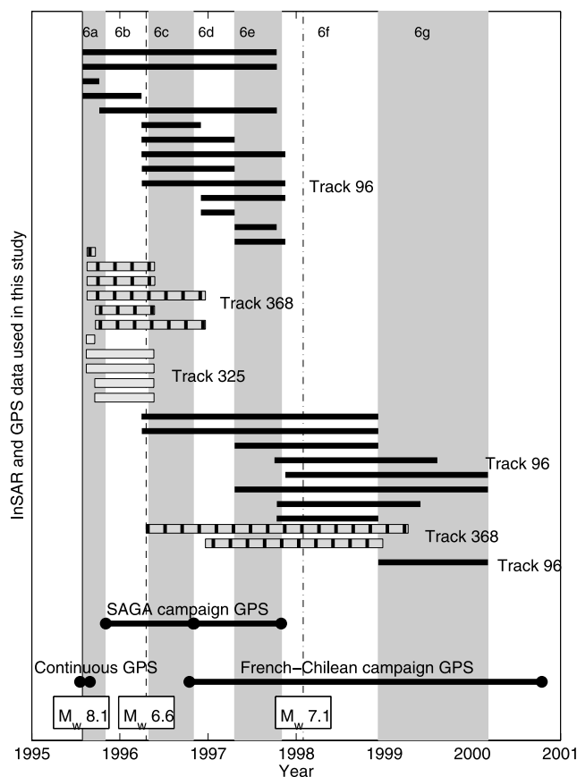
Figure 3. Time spans of geodetic data in northern Chile. Dates for InSAR images are listed in Table 1. Each different track of InSAR data is shown as a different symbol. There are three campaigns of GPS data: 3 to 15 months postseismic [Klotz et al. , 2001]; the second year postseismic (15 to 27 months postseismic) [Khazaradze and Klotz, 2003]; and between October 1996 and October 2000 (15 to 63 months postseismic) [Chlieh et al. , 2004]. Continuous GPS measurements are from a single station in Antofagasta [Melbourne et al. , 2002]. The alternating gray and white columns labeled 6a, 6b, etc., correspond to the temporal subdomains adopted in this study. The slip in each subdomain is shown in the corresponding frames of Figure 6 text, e.g., fault slip during the time interval spanned by 6a is shown in Figure 6a. We remove models of deformation from the 1996 ( M_w 6.7) and 1998 ( M_w 7.1) earthquakes [Pritchard, 2003; Pritchard et al. , 2006] from the InSAR and GPS data. It is possible that our models for the 1996 and 1998 earthquakes include some postseismic deformation (because the InSAR data spans many months/years), but these effects are small based on nonseismic interferograms and because our coseismic models for these earthquakes are also constrained by seismic data. We also remove the effects of interseismic deformation during the time periods [Bevis et al. , 2001; Khazaradze and Klotz, 2003; Chlieh et al. , 2004].
