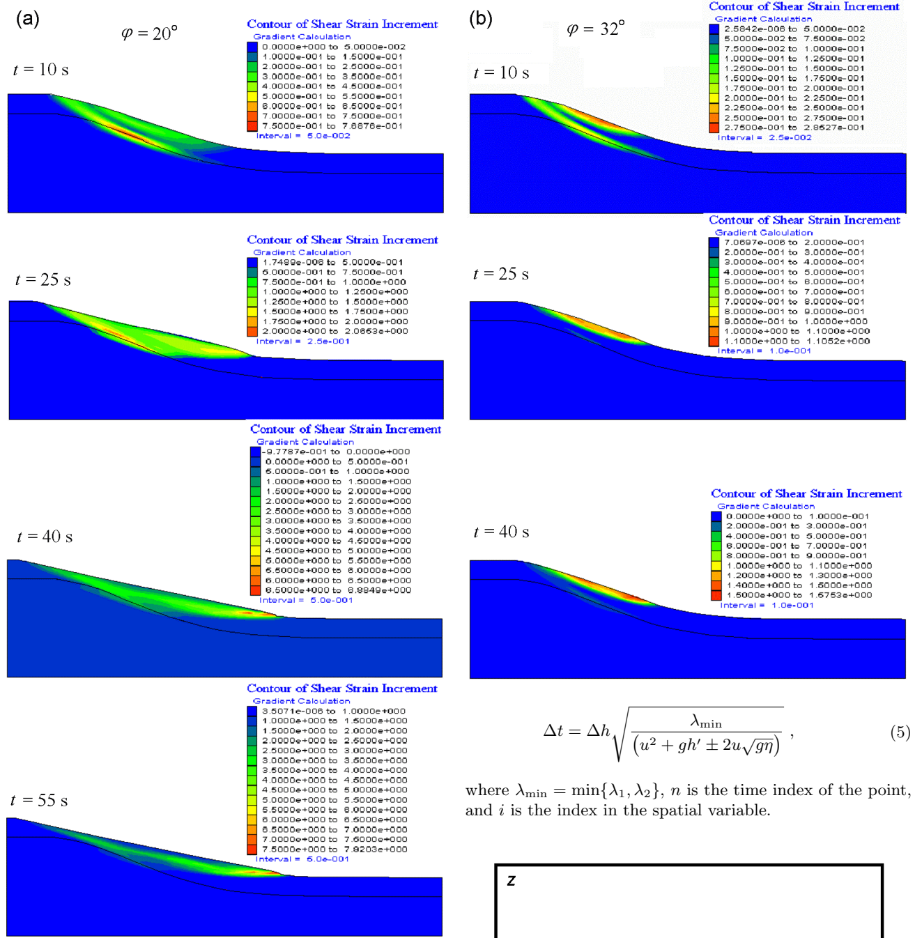
Figure 5. Distribution of the shear strain during the landslide movement computed for four time moments.
