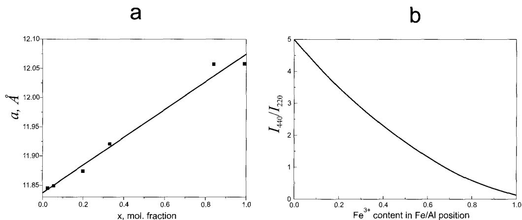
FIG. 1. (a) The lattice constant a (data taken from Novak and Gibbs, 1971; Lager et al. , 1989; Allen and Buseck, 1988) as a function of \text{Fe}^{3+} fraction x in grandite; (b) the calculated intensity ratio of 440 and 220 reflections as a function of the \text{Fe}^{3+} content in the \text{Fe}^{3+}/\text{Al} crystallographic position in the structure of grandite.
