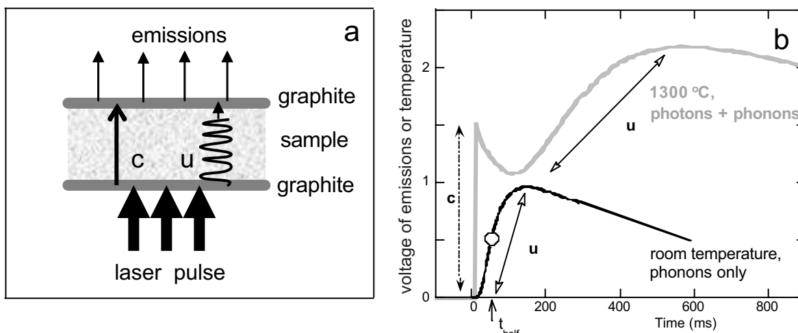
FIGURE 1. Principles of operation of a laser flash apparatus. (a) Physical transfer of heat during the experiment. A plate-shaped sample (stipple) is coated top and bottom with graphite and held at some given temperature in a furnace. Emissions (light arrows) from the top coat are recorded by an infrared detector, giving a baseline. The laser pulse (heavy arrow) is totally absorbed by the bottom graphite coat. Heat from the bottom coat then either traverses the sample as photons (medium arrow) near the speed of light ( \sim c ), or as phonons (squiggle arrow) at roughly the speed of sound ( \sim u ). For light-colored samples, essentially no absorption occurs and all radiative transfer is the boundary-to-boundary type shown here. (b) Corresponding record of heat transfer. Emissions are measured as signal voltage and set to zero before the laser pulse at t = 0 . Model curves from our experiments are shown. At low temperature (black curve), emissions are low and radiative transfer is negligible. Virtually all heat is carried by the phonons, causing the emissions (temperature) of the top graphite coat to rise gradually with time since phonons travel near sound speeds. The position for the half rise time used in analysis (Eq. 1) is shown by the circle. The result is that the peak in emissions (temperature) of the top graphite coat lags behind the laser pulse. At high temperature, radiative transfer from the bottom coat warms the top coat, giving the sharp rise in emissions almost instantaneously (schematically shown at the dotted double arrow marked “c.”) The slower phonon travel occurs afterward, indicated by the solid double arrow marked “u.” Emissions then decrease as the sample re-equilibrates with its surroundings.
