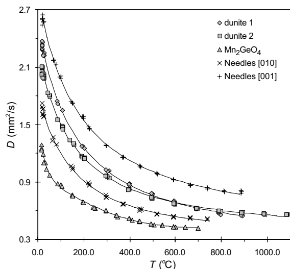
FIGURE 9. Thermal diffusivity of polycrystalline samples compared with selected oriented single crystal data. Dunites 1 and 2 have slightly different D values at room temperature, intermediate to [010] and [001] of the Needles single crystal of similar composition. The dunite 1 and 2 samples were cut at random orientations from separate hand specimens but have very similar D at high temperature. This indicates that bulk thermal diffusivity is defined by individual small crystals that exhibit a preferred orientation of [010] and [001] with no or negligible [100] or, alternatively, is dominated by [010] oriented grains with variable contributions from [001] and/or [100].
