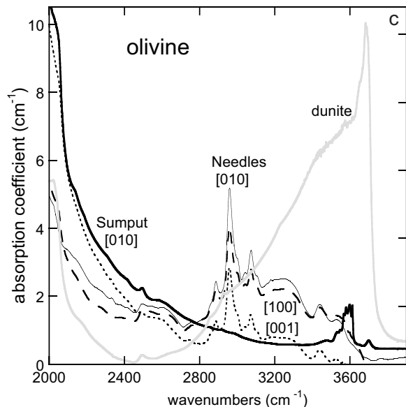
FIGURE 2. Absorption spectra of olivine analogs. (a) Sinhalite with comparison to olivine: the intense band at 900 cm -1 is due to Fe 2+ in sinhalite (black curve). The same orientation of olivine is shown as the gray dotted curve. Inset shows the O-H bands and overtones of sinhalite. Tick marks indicate peak positions. (b) Co-doped forsterite and forsterite: solid curve = [001], dotted curve = [010]. All broad bands are due to Co 2+ transitions. Inset: comparison of overtone spectra with forsterite; heavy solid curve = E||b of forsterite; gray curve = E||a of forsterite; light solid curve = [001] of Co-doped sample; dots = [010] of Co-doped sample. (c) Absorption spectra of the overtone and O-H stretching spectral regions for various forsteritic olivines. Gray curve = dunite; heavy solid curve = [010] of Sumput olivine; light curves are the three faces of Needles olivine.
