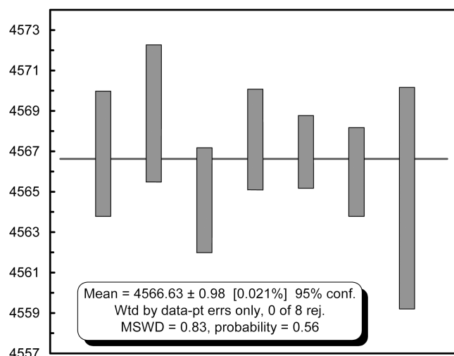
Fig. 2. Weighted average of three-point internal Pb-Pb isochrons ( \text{HNO}_3 wash, HCl wash, residue) for each of eight fractions of Allende chondrules (fractions 21–28 in Table 1). The data point for the fraction 22, with large error bar, is omitted from the figure for clarity, but is included in the weighted average calculation. Omission of this point from calculation has trivial effect on the weighted average value.
