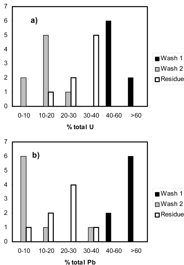
Fig. 3. Distribution of U (a) and total Pb (b) between \text{HNO}_3 leachates (Wash 1), HCl leachates (Wash 2), and residues of eight chondrule fractions analyzed during analytical session 4. The distributions for U and Pb are not identical, suggesting decoupled extraction of U and Pb. These results show that over 50% of U and Pb in chondrules are relatively poorly bound and are extracted during the first leaching step.
