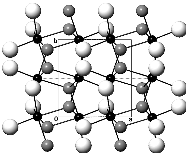
FIG. 1. Projection of the crystal structure of arsenopyrite from La Roche-Baluc along the c axis. Black, grey and white circles refer to Fe, As and S atoms, respectively. Stippled and dashed lines: long and short Fe-Fe bonds, respectively.
