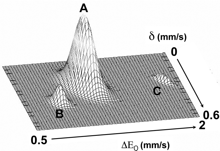
FIG. 5. Two-dimensional site distribution of isomer shift \delta versus quadrupole splitting \Delta E_Q of the Mössbauer spectrum for arsenopyrite from La Roche-Balue.
