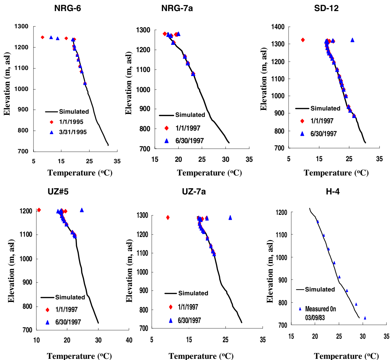
Fig. 13 Comparisons between measured and simulated ambient temperature profiles for six boreholes under the present-day mean infiltration rate
