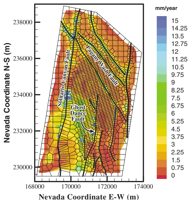
Fig. 10 Simulated percolation fluxes at the water table, using the present-day mean infiltration scenario of the base-case model results (preq_mA)
