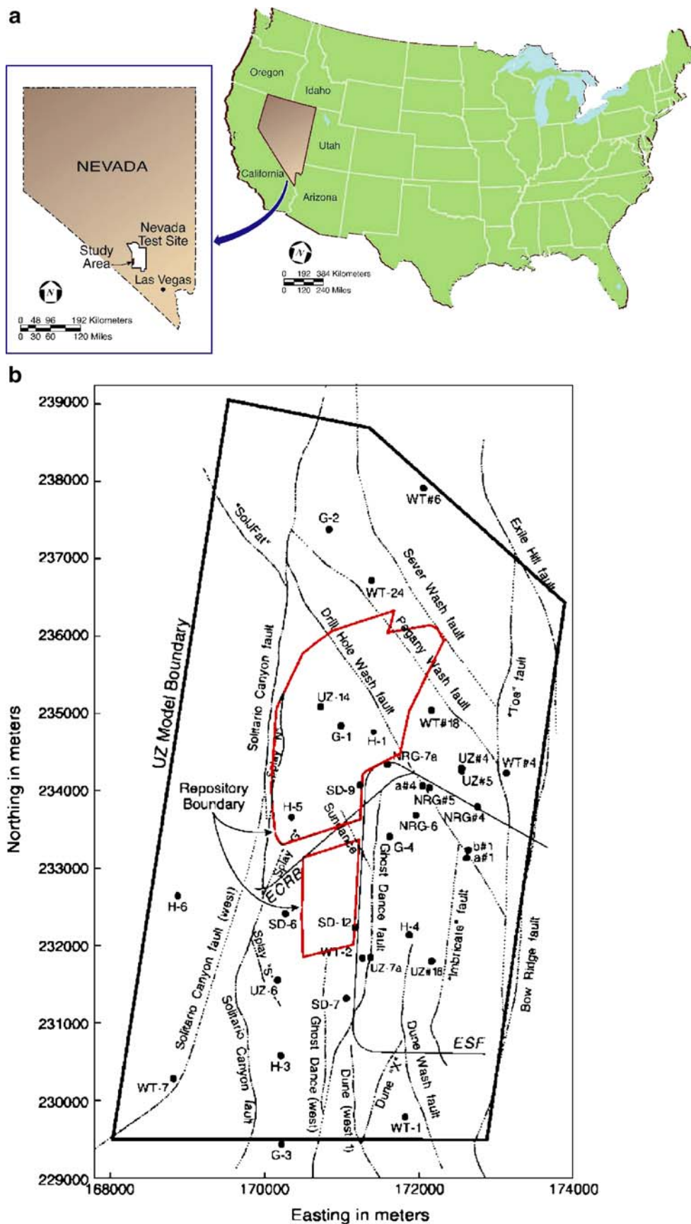
Fig. 1 a Location of Yucca Mountain study site, USA, b Plan view of the UZ model domain, showing the model boundary, the potential repository outline (in red), major fault locations, the paths of the ESF (Exploratory Studies Facilities) and ECRB (Enhanced Characterization of Repository Block) tunnels, and selected borehole locations
