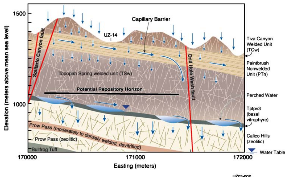
Fig. 2 Schematic showing the conceptualized flow processes and effects of capillary barriers, major faults, and perched-water zones within a typical east-west cross section of the UZ flow model domain (modified from Zhang et al. 2006)
