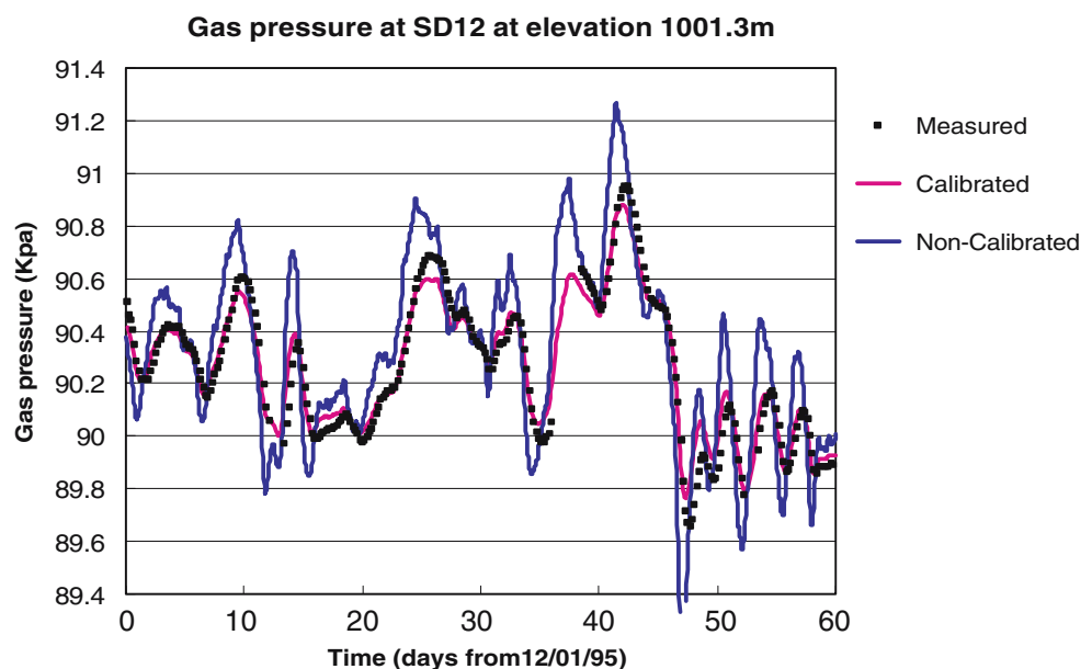
Fig. 5 Comparison of simulated and observed gas pressures at borehole SD-12 during a 60-day period, using simulation results with and without three-dimensional calibration
