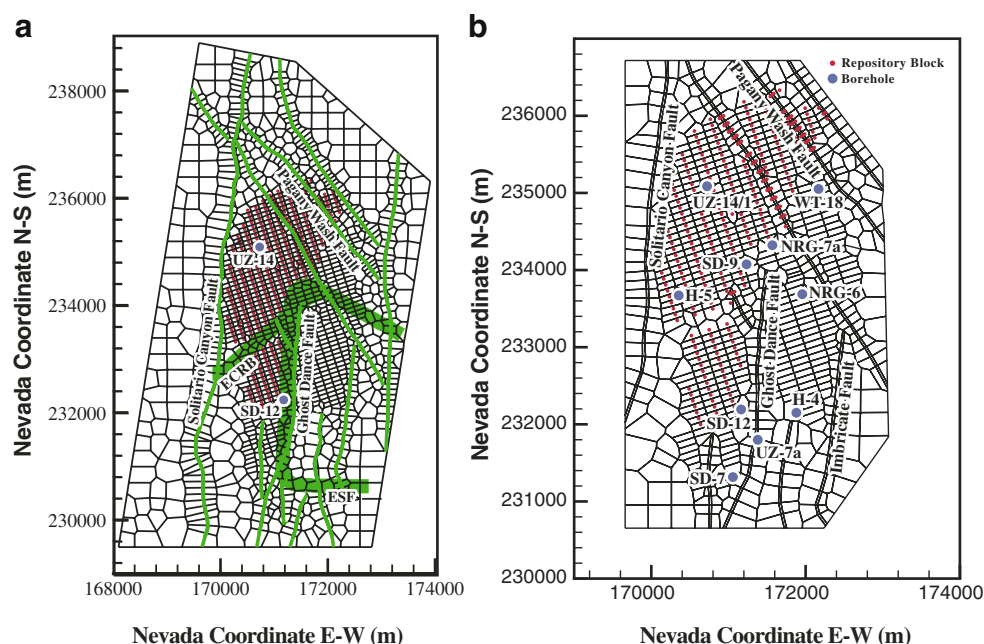
Fig. 3 a Plan view of the three-dimensional UZ flow model grid, showing the model domain, faults incorporated, repository layout, and several borehole locations (modified from BSC 2004). b Plan view of the three-dimensional thermal model grid showing a smaller model domain, used for modeling gas and heat flow
