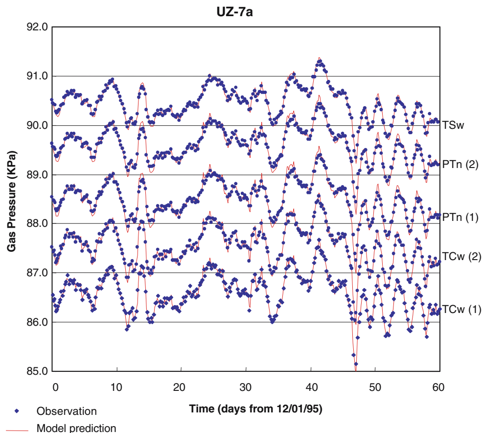
Fig. 6 Comparison of simulated and observed gas pressure at borehole UZ-7a over a 60-day period. (There are five observations in total: two observations are located at TCw , two observations are located at PTn , and one observation is located at TSw )
