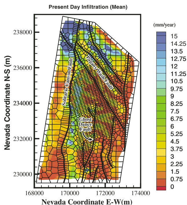
Fig. 4 Plan view of net infiltration distributed over the three-dimensional UZ flow model grid for the present-day (base-case) mean infiltration scenario (modified from Wu et al. 2004)
