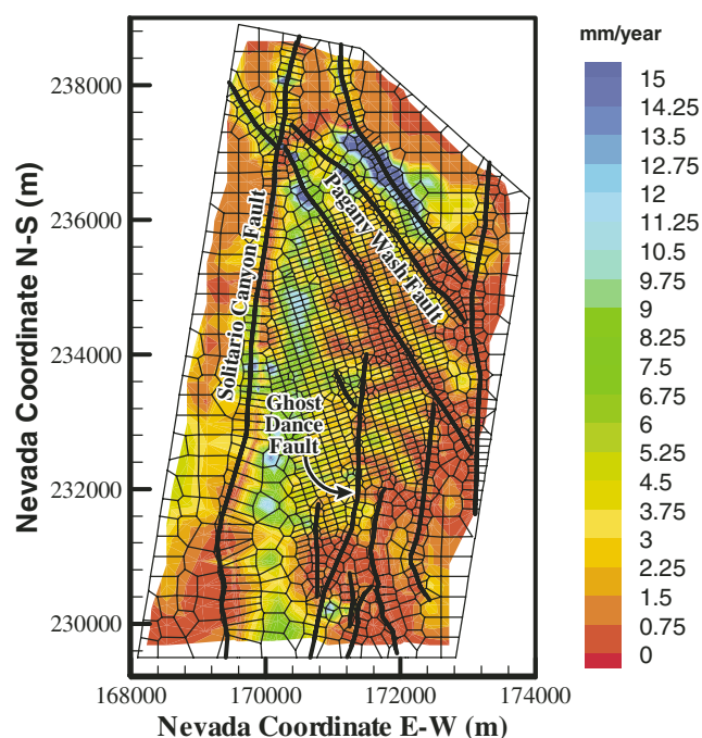
Fig. 8 Simulated percolation fluxes at the repository horizon, using the present-day mean infiltration scenario, alternative model results (preq_mB)
