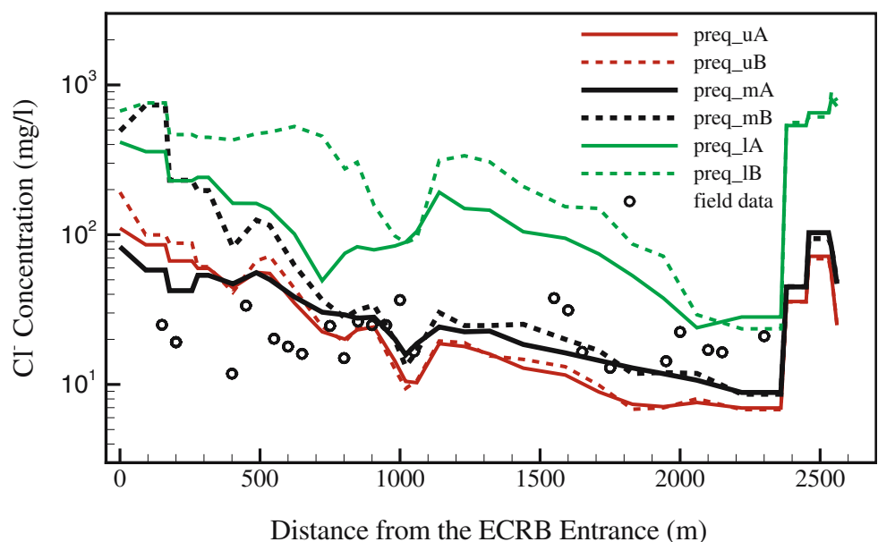
Fig. 14 Comparison between measured and simulated chloride concentration (mg/l) profiles along the ECRB (Enhanced Characterization of Repository Block) tunnel for present infiltration with mean, upper, and lower bound
