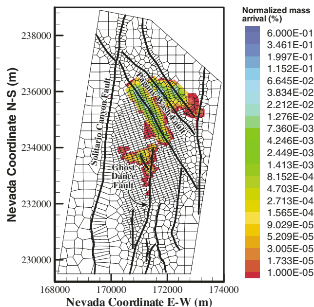
Fig. 12 Simulated cumulative, normalized mass-arrival contours of a reactive tracer at the water table after 1,000 years, identifying potential breakthrough areas, using the present-day mean infiltration scenario of the base-case model
