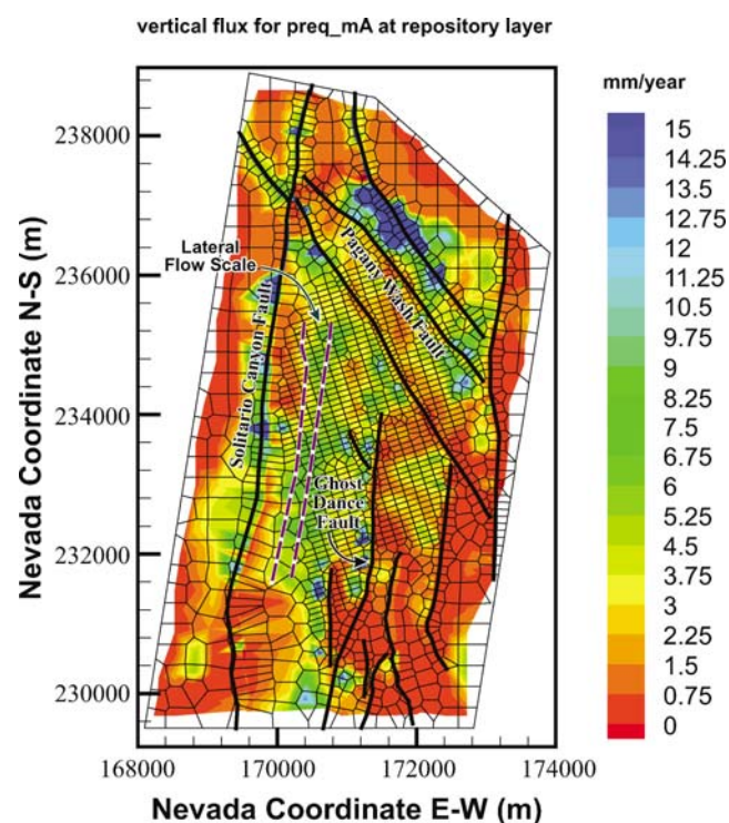
Fig. 7 Simulated percolation fluxes at the repository horizon, using the present-day mean infiltration scenario, base-case model results (preq_mA; modified from Wu et al. 2004)
