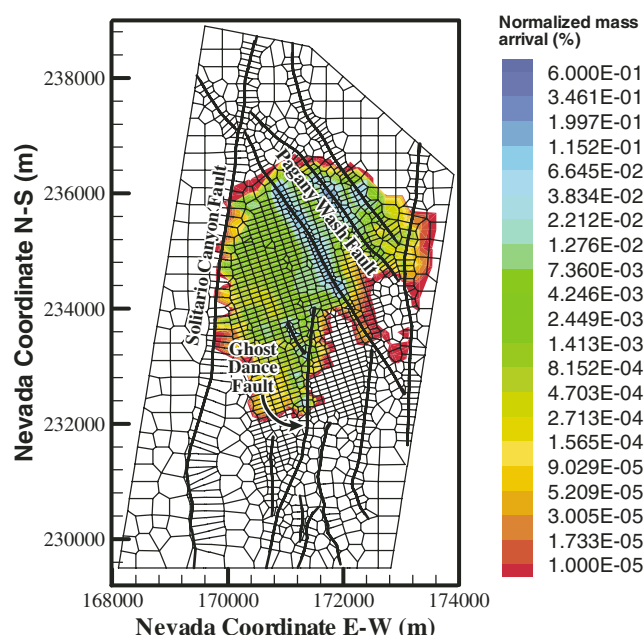
Fig. 11 Simulated cumulative, normalized mass-arrival contours of a conservative tracer at the water table after 1,000 years, identifying potential breakthrough areas, using the present-day mean infiltration scenario of the base-case model
