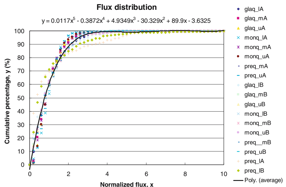
Fig. 9 Cumulative flux distribution and range (as functions of normalized percolation flux within the repository) from the 18 flow fields (equation is valid for 0.05 < x < 10 , with x being normalized flux, and y being cumulative area percentage)
