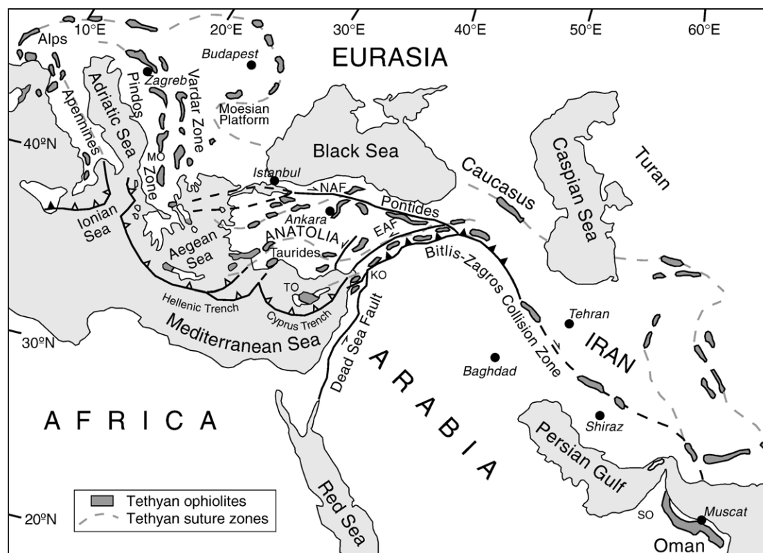
Fig. 1. Simplified tectonic map of the eastern Mediterranean region showing the distribution of the Neotethyan ophiolites and suture zones. Key to lettering: MO — Mirdita ophiolites, KO — Kizildag ophiolite, SO — Semail ophiolite, TO — Troodos ophiolite.
