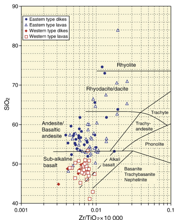
Fig. 9. Geochemical classification of the lavas and dikes from the Western- and Eastern-type ophiolites using the \text{Zr}/\text{TiO}_2 \times 10,000 versus \text{SiO}_2 diagram of Winchester and Floyd (1977).
