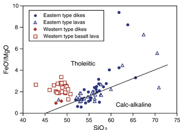
Fig. 8. \text{SiO}_2 versus \text{FeO}/\text{MgO} diagram of the lavas and dikes from the Western- and Eastern-type ophiolites. The boundary between tholeiitic and calc-alkaline rock types is from Miyashiro (1974). Some of the lava flows of the upper part of the volcanic sequence of the Eastern ophiolites contain quartz-bearing amygdals, and in some of the samples (lavas and dikes of both WO and EO) there are thin quartz-filled fractures. We have avoided these samples in the diagram.
