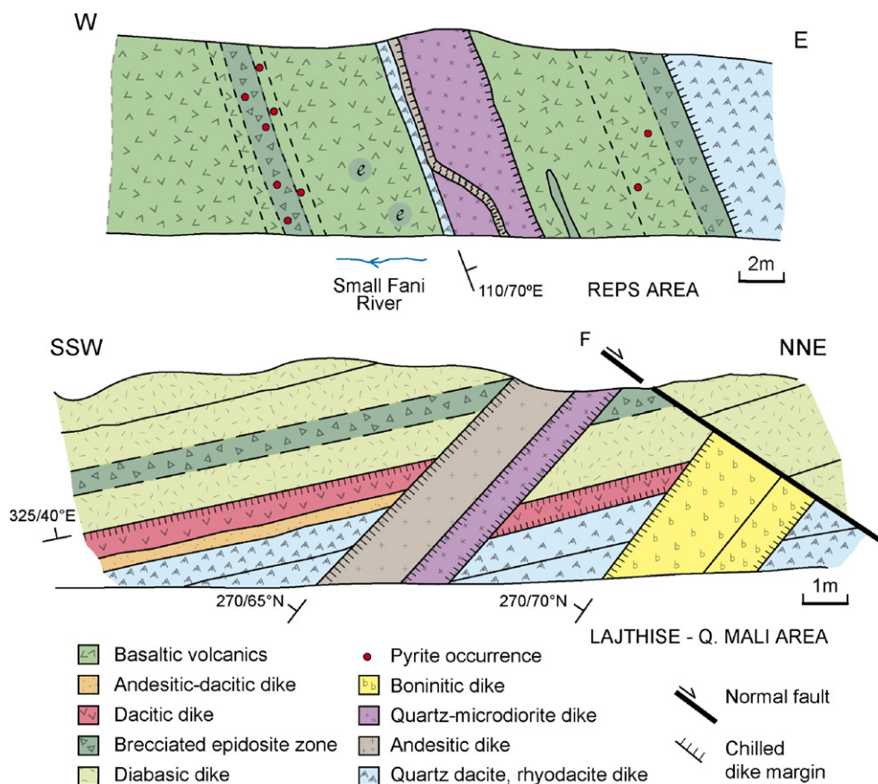
Fig. 7. Roadcut sections of the sheeted dike complex of the Eastern-type ophiolites in the Repts (A) and Lajthiș-Q. Mali (B) areas. These locations are marked on Fig. 4.
