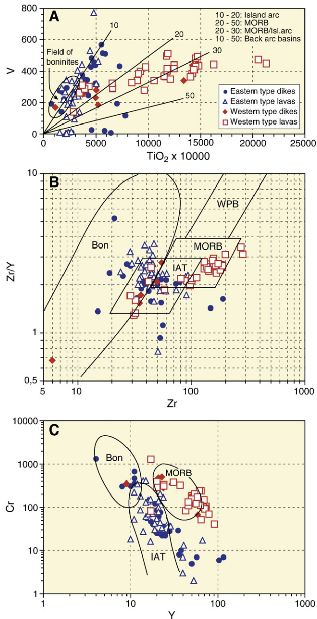
Fig. 10. \text{TiO}_2 –V (A), \text{Zr} – \text{Zr}/\text{Y} (B), and \text{Y} –Cr (C) discriminant diagrams. MORB=mid-ocean ridge basalts, IAT=island arc tholeiites, WPB=within-plate basalts, Bon=boninites. See Pearce (2003) for further references to these discriminant diagrams.
