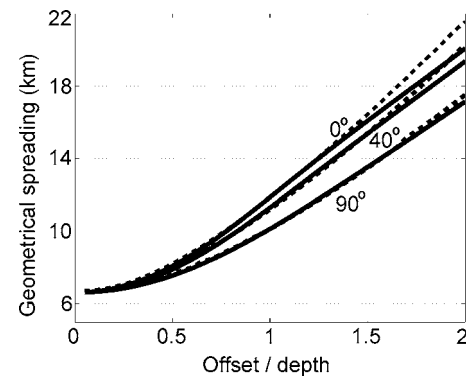
Figure 9. Accuracy of our method for the reflection from the bottom of layer 3 in model 1; the azimuths from the [x_1, x_3] symmetry plane are \alpha = 0^\circ , 40^\circ , and 90^\circ . The geometrical-spreading factor L computed by our algorithm (solid lines) is compared with the output of dynamic ray-tracing code ANRAY (dashed).
