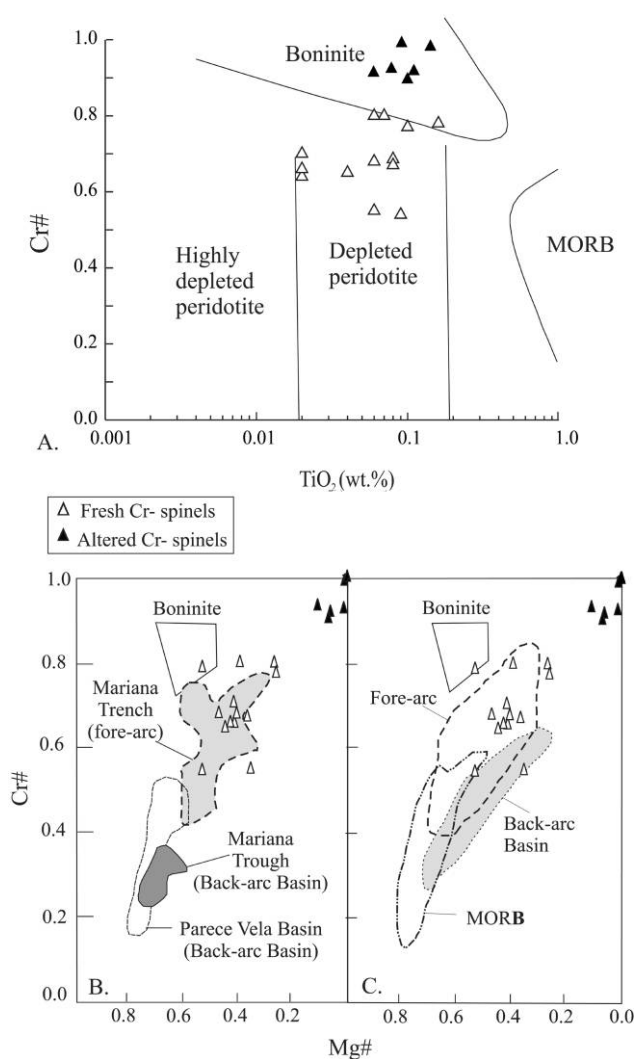
Figure 6. A, Cr# versus TiO 2 diagram for the analyzed accessory chrome spinels (fields after Dick and Bullen 1984; Jan and Windley 1990; Arai 1992). B, Cr# versus Mg# for the analyzed spinels and their alteration products (modified by Proenza et al. 2004; after Dick and Bullen 1984). C, Cr# versus Mg# for the analyzed spinels and their alteration products (adopted from Stern et al. 2004). MORB = mid-ocean ridge basalt.
