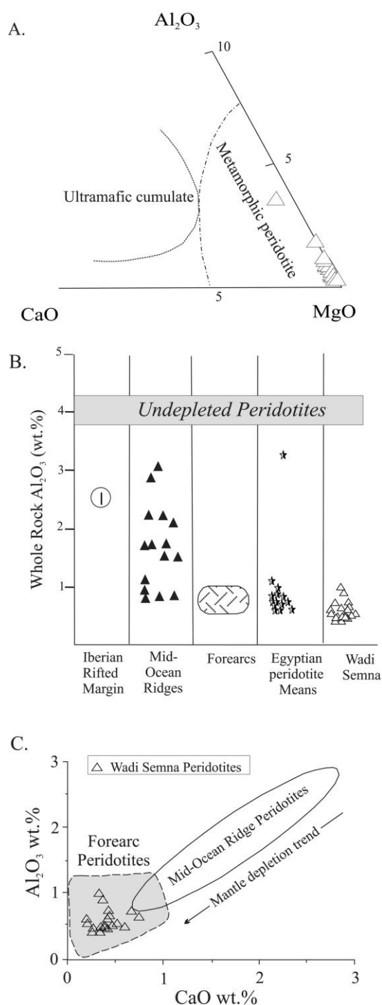
Figure 3. A, \text{Al}_2\text{O}_3 - \text{MgO} - \text{CaO} diagram for the studied serpentinites (Coleman 1977). B, Whole-rock \text{Al}_2\text{O}_3 content in Wadi Semna serpentinites and other Egyptian Neoproterozoic peridotites compared with peridotites from other tectonic settings (modified after Bonatti and Michael 1989). The means of different localities in the Eastern Desert of Egypt are calculated on the basis of data
