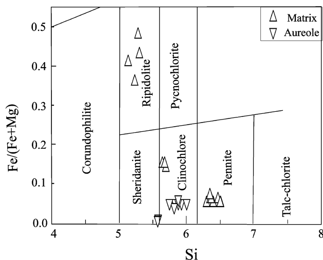
Figure 5. Chlorites in Wadi Semna serpentinites. Note Fe-poor nature of chlorites in aureoles around altered spinels. Fields after Hey (1954).
