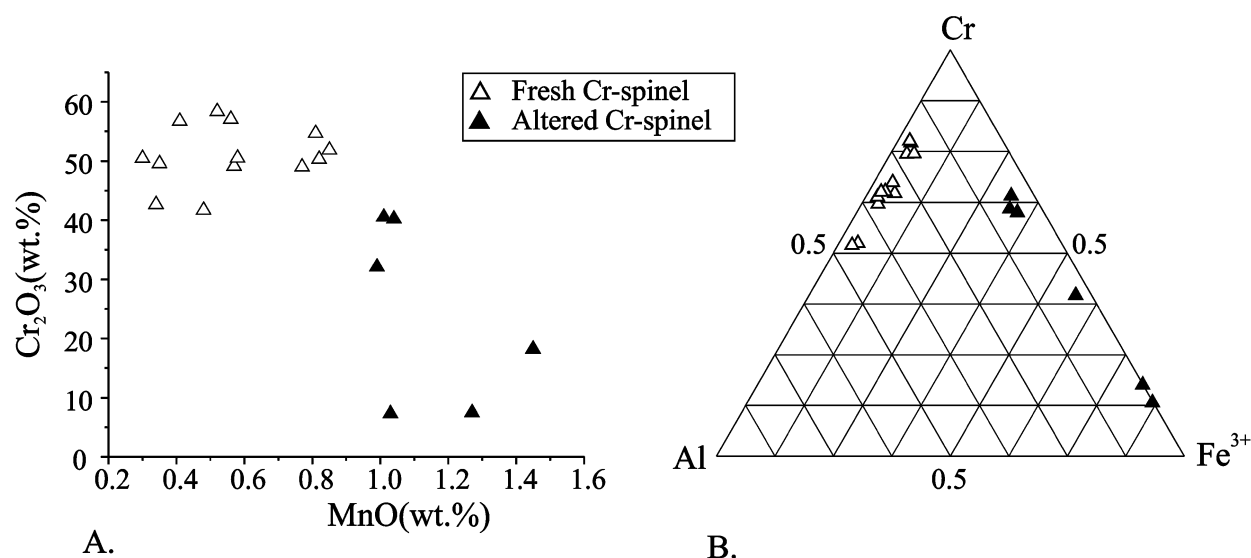
Figure 4. Fresh and altered Cr spinels in Wadi Semna serpentinites. A, \text{Cr}_2\text{O}_3 versus MnO plot of fresh (Mn-poor) and altered (Mn-rich) chrome spinels. B, Cr-Al- \text{Fe}^{3+} plot of Wadi Semna chrome spinels and their Al-poor alteration products.
