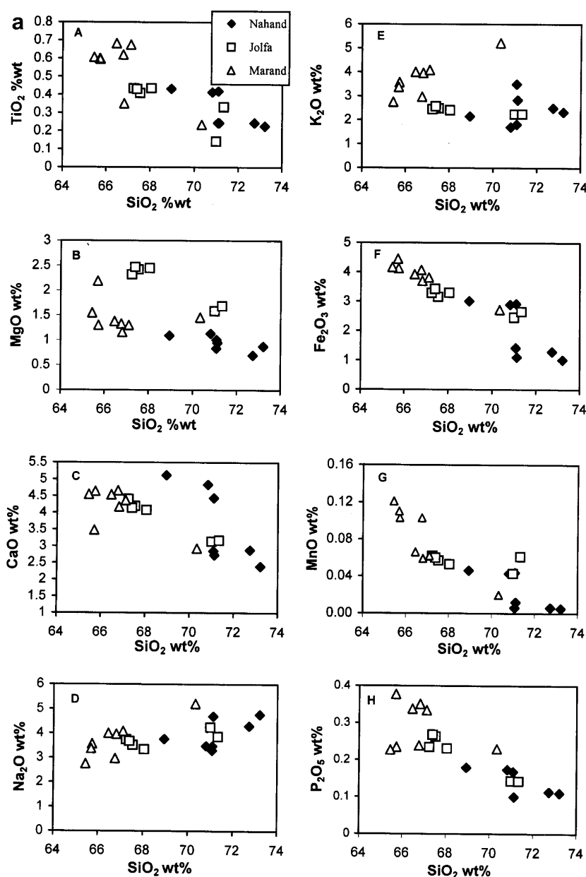
Fig. 8. Variation diagrams for major and trace elements of dacitic and rhyodacitic rocks of NW Iran. Major and trace elements are in wt% and ppm, respectively. \text{Fe}_2\text{O}_3 as \text{Fe}_2\text{O}_3 total.
