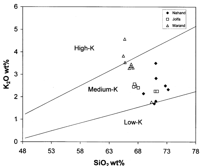
Fig. 9. \text{SiO}_2 vs. \text{K}_2\text{O} for dacitic rocks of NW Iran. Most of the samples plot in the medium-K field. High-K samples suspected of crustal contamination.
