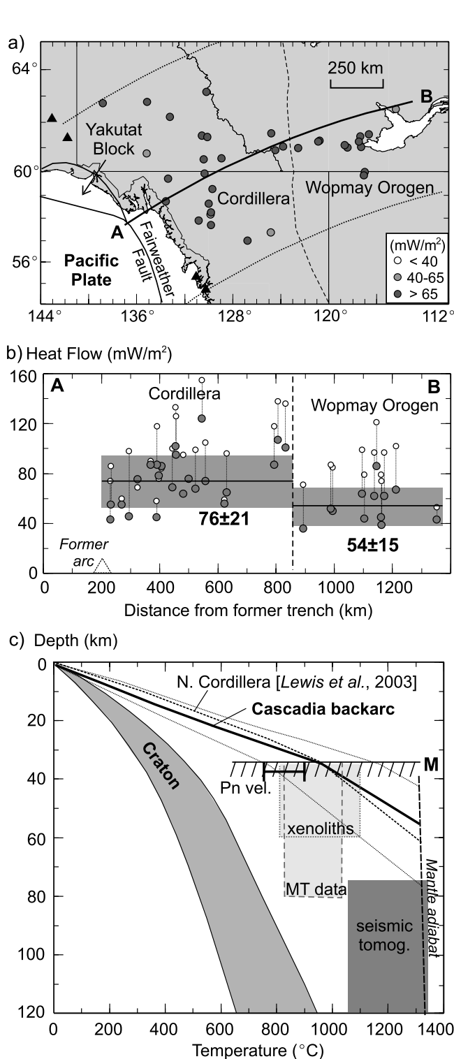
Figure 13. (a) Heat flow data for the Northern Canadian Cordillera. Subduction along this margin ceased at \sim 42 Ma. (b) Heat flow profile. The original heat flow values (open circles) have been corrected for variations in upper crustal heat production (solid circles) (see text). (c) Observational constraints on thermal structure. The dashed line is the geotherm from Lewis et al. [2003]. The Cascadia back arc and Archean craton geotherms are shown for comparison.
