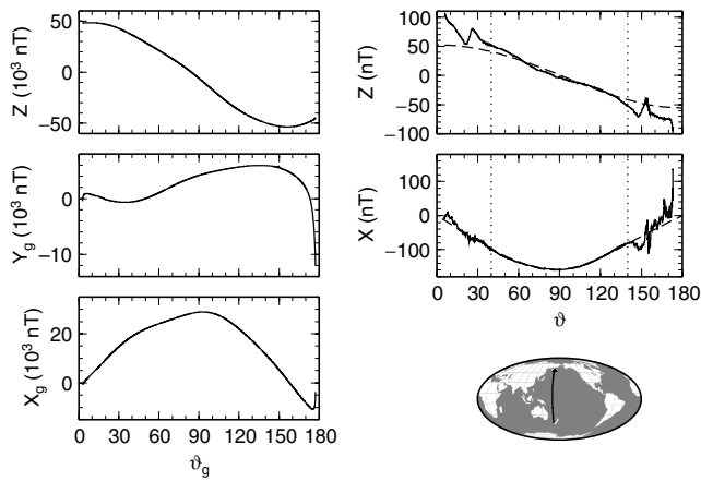
Figure 1. CHAMP satellite data from track 18968 (arrow on global map insert), which samples the relaxation phase of storm 11 above the Pacific Ocean. Left plates: The original CHAMP data plotted along geographic colatitude \vartheta_g . X_g , Y_g and Z components point, respectively, to the geographic north, east and downwards. Right plates: Solid lines denote the CHAMP ( X , Z ) data after removal of the comprehensive model, rotation into dipole coordinates and removal of a constant shift from the Z component. Dashed lines show the results of the two-step spherical harmonic analysis, including the extrapolation in the polar areas. For this particular track we use data from the colatitude interval ( 40^\circ , 140^\circ ), as marked by dotted lines.
