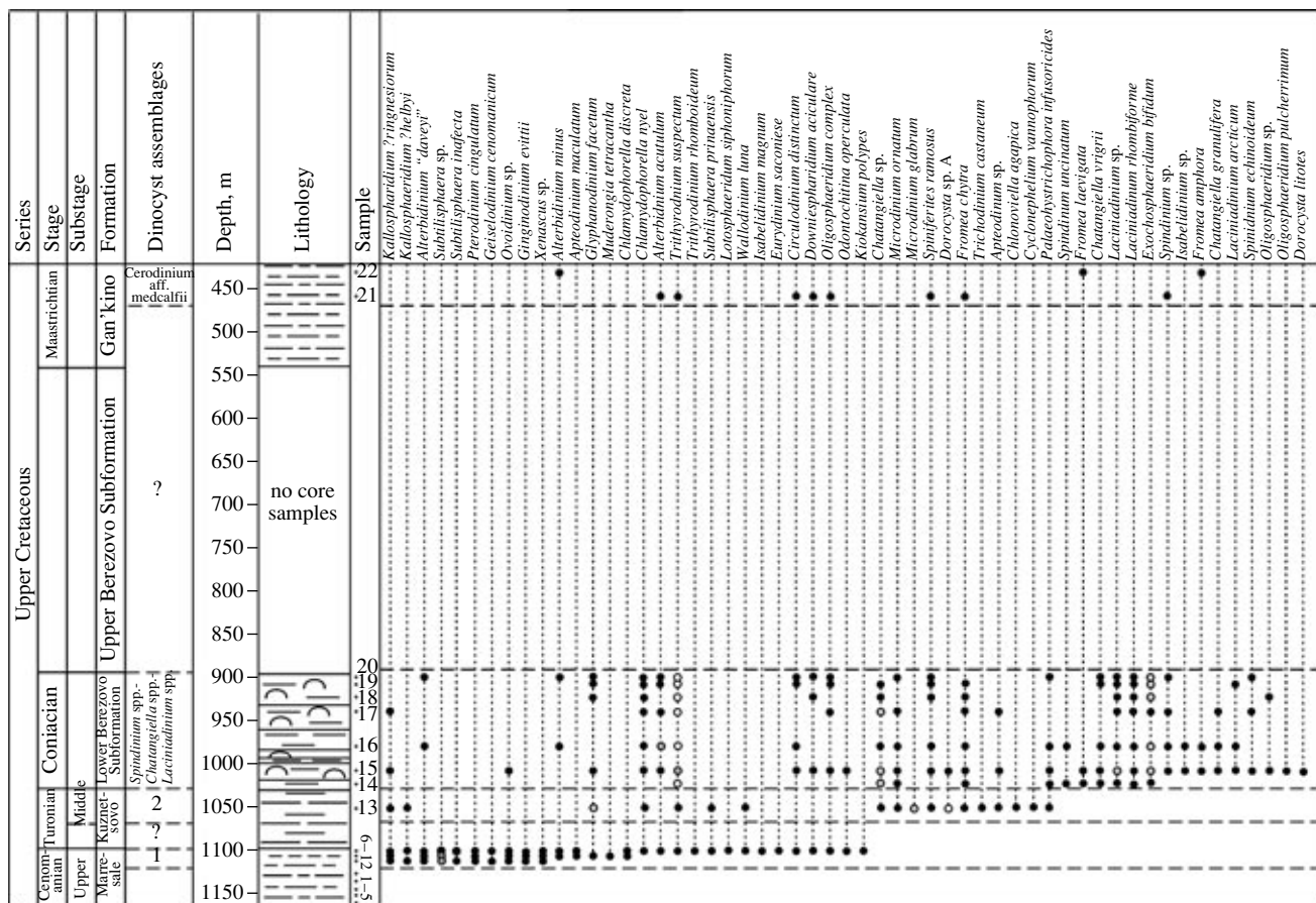
Fig. 4. Stratigraphic ranges of dinocysts in the Upper Cretaceous section of borehole Leningradsкая 1. Designations: (1) assemblage with Eurydinium saxoniense Marshall et Batten; (2) assemblage with Dorocysta sp. A; (Lower Berez.) Lower Berezovo Subformation; (Kuz.) Kuznetsovo (Mid.) Middle; ( Spiniferites ram. ) Spiniferites ramosus ; for other designations, see Figs. 2 and 3.
