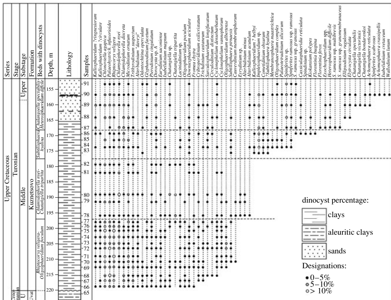
Fig. 2. Stratigraphic range of dinocysts in the Upper Cretaceous section of borehole Berezovskaya 23k. Designations: ( Palaeohystrich. ) Palaeohystrichophora ; ( S. ) Spiniferites .
