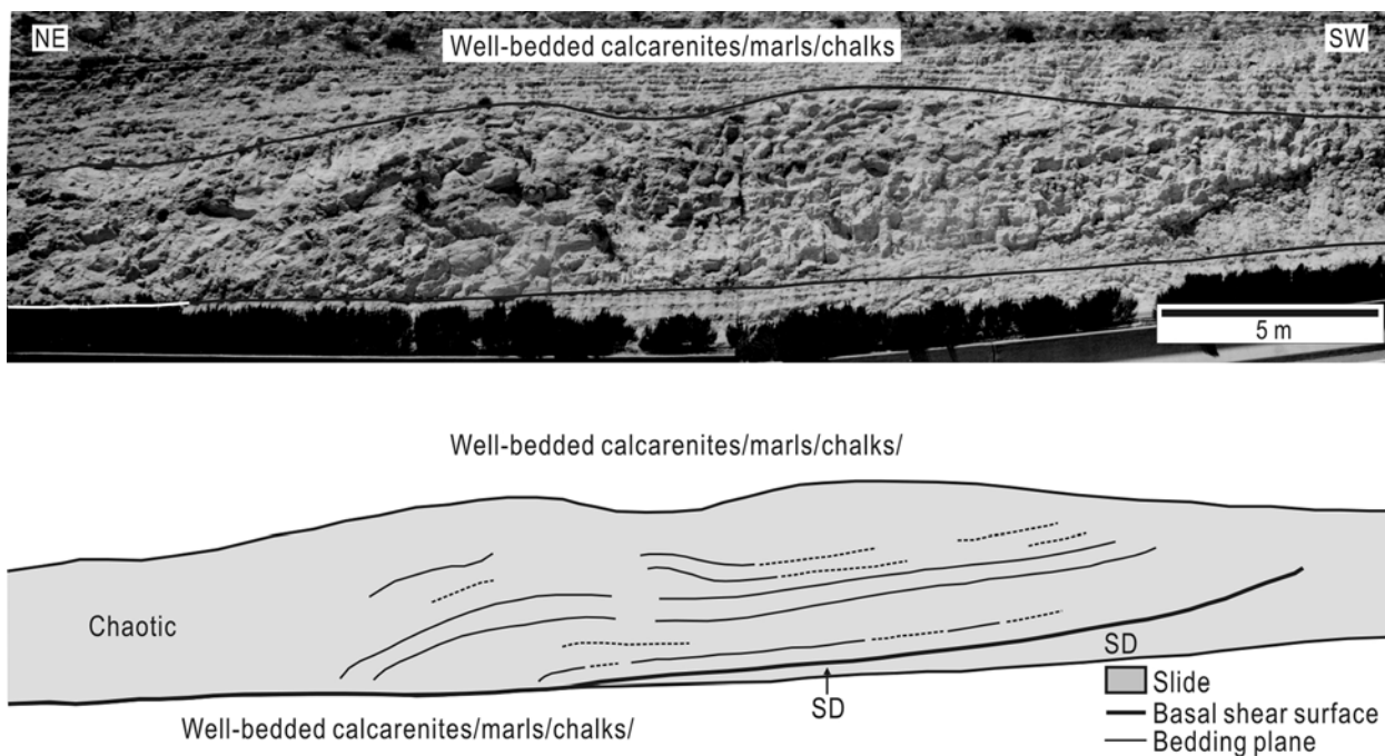
Fig. 4. Photograph (top) and line drawing (bottom) displaying sedimentary features of submarine landslide deposits (Section 3). Note a slightly rugged morphology of the upper surface and a tangentially curved geometry of the basal shear surface at end of the flat portion. SD in the bottom indicates a severe or intense deformation. For location of the section, see Fig. 1B.
