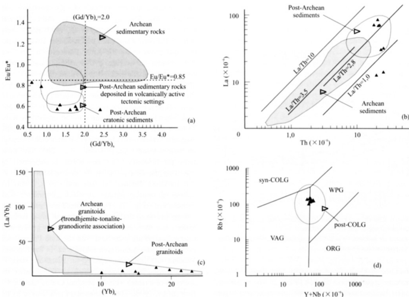
Fig. 8. Data on metapelites of the Korda Formation (black triangles) reported in the different plots and diagrams.
