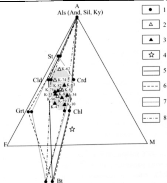
Fig. 4. AFM phase diagram (Thompson, 1957) representing the chemical compositions of rocks and minerals, and typical mineral assemblages of Fe- and Al-rich metapelites.
