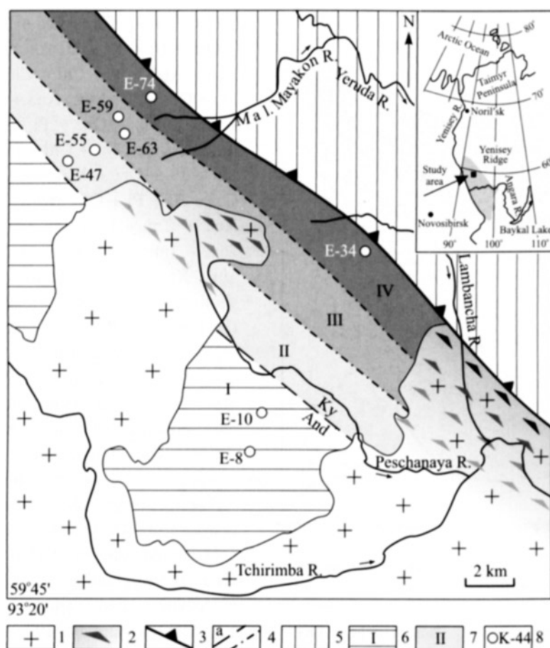
Fig. 3. A geological sketch map of collisional metamorphism on the eastern margin of the central part of the Transsiberian region of the Yenisey Ridge in the vicinity of the Panimba thrust.
