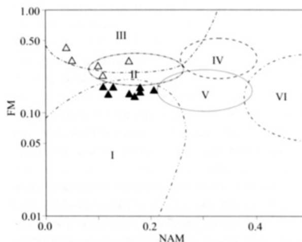
Fig. 5. Data points of Amar Formation (open triangles) and Korda Formation (black triangles) metapelites plotted in the FM-NAM module diagram (Yudovich and Ketris, 2000).
