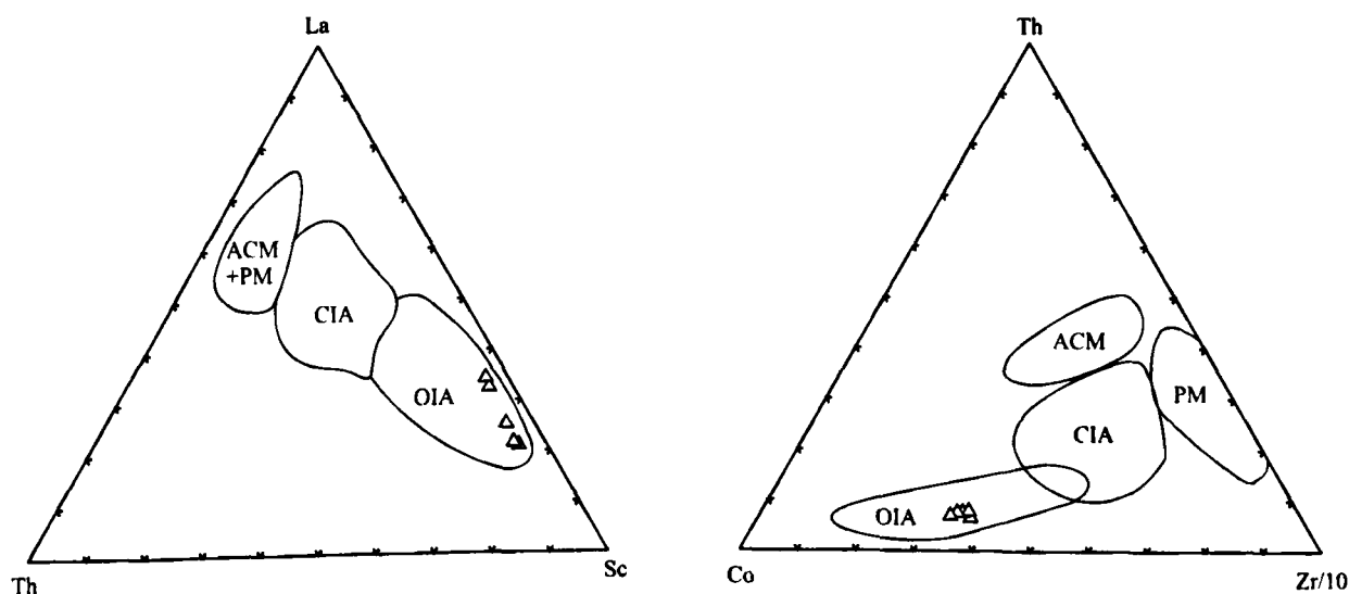
Fig. 7. Data on metapelites of the Amar Formation (open triangles) plotted in Th-Co-Zr and La-Th-Sc ternary diagrams for tectonic discrimination of graywackes (Bhatia and Crook, 1986).
