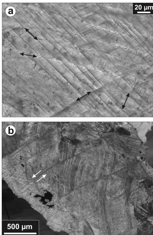
Fig. 11. Microphotographs of calcite grains. a) Grains with anomalous number of microfeatures (twins, cleavages, or planar fractures? Up to 4 different orientations). Suevite sample KR8-006; depth = 240.36 m (plane-polarized light). b) Grains with fractures, microfaults, and curved twins. Meta-graywacke sample KR8-108; depth = 424.78 m (cross-polarized light).
