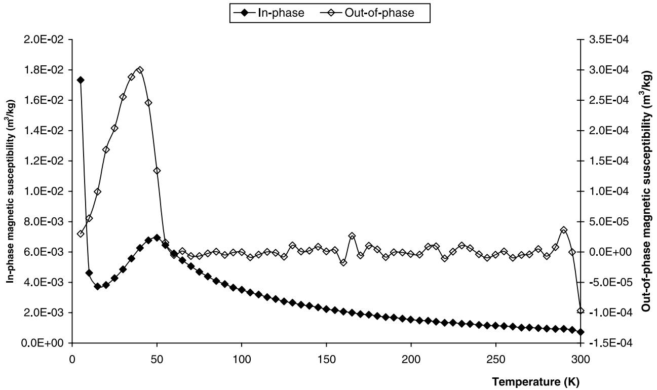
Figure 8. Temperature dependence of in-phase and out-of-phase magnetic susceptibility of amorphous Fe 2 O 3 [Zbořil et al. , 2004]. Decrease of the latter parameter to zero at 55 K reflects that the onset of paramagnetic behavior (absence of the minor hysteresis loop area) corresponds well with the onset of hyperbolic decay on the in-phase susceptibility.
