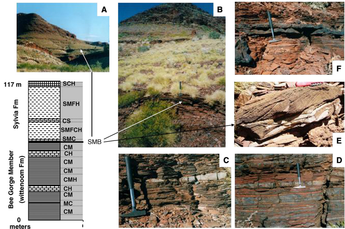
Fig. 6. Bee Gorge section (see Fig. 5 for location). Columnar section and outcrops of the Bee Gorge Member (BGM) of the Wittenoorn Formation, Spherule Marker Bed (SMB) and Mount Sylvania Formation; C – carbonate; M – marl and calcareous siltstone; H – chert; S – siltstone; F – ferruginous siltstone and chert. (A) A view of Bee Gorge Creek section east of the opening of Bee Gorge. Arrow points to the location of the SMB. (B) Outcrop of the SMB overlain by siltstone, ferruginous siltstone and minor carbonate. The brown bank at mid-distance is the uppermost carbonate unit in the section, overlain by ferruginous siltstone and Fe–chert. (C) Bee Gorge Member: calcareous siltstone (marl) including a carbonate layer (white). (D) Bee Gorge Member: carbonates (grey layers) and calcareous siltstone (red). (E) SMB: microkrystite spherule-bearing cross layered turbidite. (F) Mount Sylvania Formation: Fe–chert layers (black) within ferruginous siltstone.
