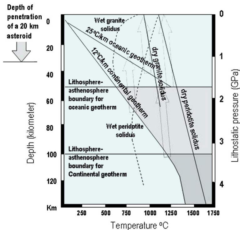
Fig. 9. Pressure–temperature diagram portraying the position of the lithosphere–asthenosphere boundary for continental and oceanic geotherms and the position of dry and wet peridotite solidi [13]. Downward arrow marks the \sim 30 km penetration depth of a 20 km asteroid, equivalent to decompression. Upward arrows mark alternative adiabatic melting paths of mantle diapirs (adiabatic cooling 0.33 \text{ }^\circ\text{C/km} ).
