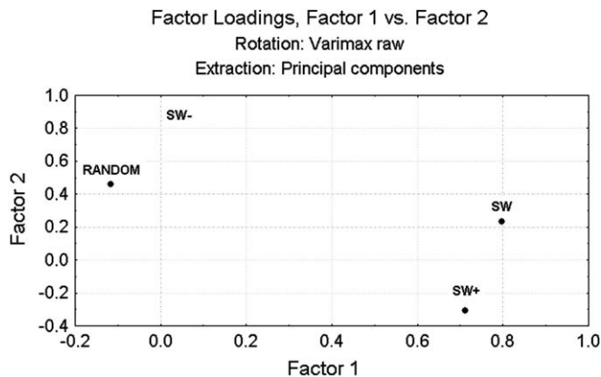
Fig. 4. Factor loadings for the variables SW, SW+, SW- and RANDOM (see text).
