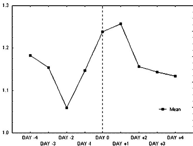
Fig. 3. Average daily number of earthquakes on days with high speed solar wind (day 0), one day before and after the arrival of high speed solar wind (day -1 and +1, respectively), etc.
