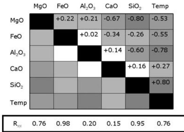
Figure 5. Resulting correlations and resolution associated with the simultaneous inversion of temperature and composition. The a posteriori covariance matrix is not diagonal indicating trade-offs between the model parameters. Their amplitudes are depicted by the grey scaling and we also show values that are greater (or lower) than 0.1 (−0.1). It indicates that there exist a family of models that will explain equally the observables used for our inversion. R_{xx} are the diagonal elements of the resolution matrix. When R_{xx} is close to 1, the parameter is well resolved, on the contrary, values close to 0 indicates the impossibility to obtain robust conclusions.
