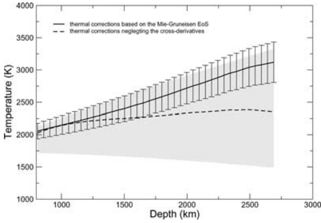
Figure A1. The influence of the extrapolation method of bulk modulus on the best-fitting geotherms when density \rho and bulk sound velocity V_\phi are being matched by the inversion. The thermal corrections obtained from a Mie-Grüneisen EoS (solid line) yield geotherms with larger temperature gradient compared to high-temperature finite-strain thermal corrections when neglecting the cross-derivatives of the incompressibility (dashed line). The temperature difference exceeds the a posteriori uncertainties below the depth 1500 km and can be as large as 700 K at the depth of 2700 K in the case of the chondritic composition. The a priori geotherm by Brown & Shankland (1981) and a priori Gaussian bounds changing linearly from \pm 200 K at 800 km to \pm 1000 K at 2700 km are depicted by the grey shading.
