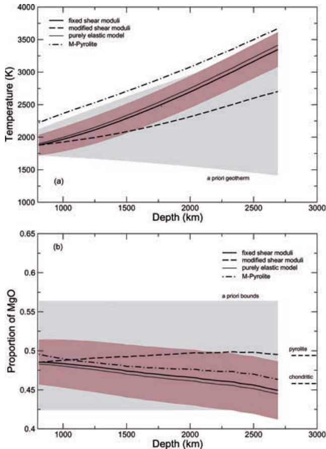
Figure 4. Resulting geotherms (a) and proportions of MgO (b), SiO 2 (c), and FeO (d) when solving simultaneously for temperature and composition. The results when the pyrolitic model is used as initial guess are denoted by solid lines. The effect of anelasticity (light-solid line) is within the a posteriori uncertainties (dark shading). The results for modified pyrolite are depicted by dot-dashed lines. The optimized composition is characterized by a decreasing Mg/Si ratio (from 1.18 to 1.03), increasing FeO content, and a geotherm having larger temperature gradient than the Brown and Shankland's geotherm. In order to improve the fit, the inversion decreases the value \mu'_0 of perovskite when the shear properties are allowed to be modified. The best matching value is 1.59 or 1.66 \pm 0.08 (see Table 4). In this case, the results are denoted by the dashed lines. The resulting geotherm is closer to the Brown and Shankland's initial profile. The Mg/Si ratio is increasing with depth (from 1.18 to 1.26), FeO content is constant with depth. The light shading denotes the initial Gaussian bounds on the temperature and compositional parameters. The proportions of Al 2 O 3 and CaO are not shown because they are only poorly resolved.
