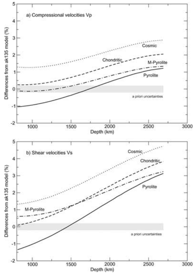
Figure 1. Differences between predicted and observed seismic velocities V_p (a) and V_s (b) for a lower mantle having uniform bulk composition model together with the Brown and Shankland's geotherm: pyrolite (solid line), modified pyrolite (dot-dashed line), chondritic model (dashed line), cosmic model (dotted line). The predicted velocities are always higher than those given by ak135, except for the top 400 km when the pyrolitic model is used. The discrepancy increases with depth and reaches 3 and 4 per cent for V_p and V_s , respectively, in the bottom of the lower mantle. The predicted discrepancies are significantly larger than the uncertainties on the radial seismic profiles (denoted by the shaded areas).
