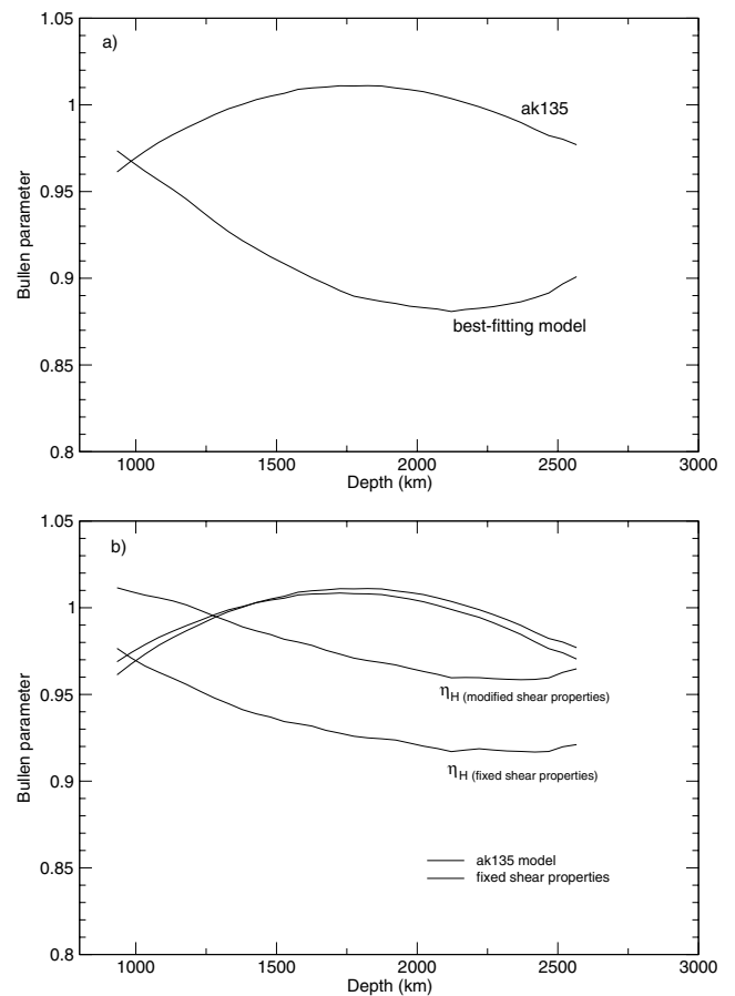
Figure 3. Bullen parameter as a function of depth. (a) Assuming uniform pyrolite (or chondritic) composition, values of the Bullen parameter are significantly lower from those obtained for ak135 below the depth of 1000 km. (b) For inversions with depth dependent bulk composition with fixed shear properties, the resulting values of \eta (solid line) matches the values obtained from ak135 (dashed line) within \pm 1 per cent. The values of \eta_H (dot-dashed line) are, however, always lower, varying between 0.97 and 0.92, than those of \eta . When the shear properties are allowed to vary, the resulting \eta matches \eta of ak135 perfectly. In this case, \eta_H (dotted line) is decreasing with depth: it is higher than 1 down to 1200 km and reaches 0.97 in the bottom of the lower mantle.
