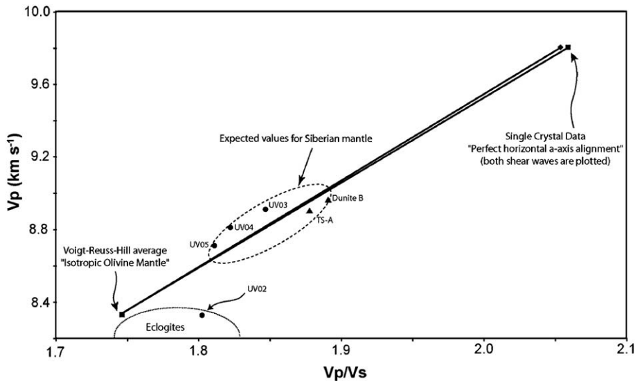
Fig. 6. V_p/V_s versus compressional wave velocity parallel to olivine [100] for increasing crystallographic orientation. The lines represent the gradient between isotropic olivine aggregate and an olivine single crystal. Real V_p and V_p/V_s values must lie somewhere in between, as shown. The separation between the lines is shear-wave anisotropy parallel to olivine [100]. Data points “TS-A” and “Dunite B” are from Christensen (1966) and Christensen and Ramanantoandro (1971), respectively. Samples UV03, UV04, and UV05 are plotted based on velocities from calculations, and sample UV02 is based off of high-pressure experimental data. The eclogite field is from average eclogite data ( \pm \sigma ) of Christensen (1996). All velocities have been adjusted for conditions of 1500 MPa and 500 °C.
