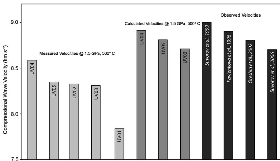
Fig. 5. Compressional wave velocities for the Udachnaya xenoliths at elevated pressures and temperatures and observations of compressional wave velocities in Siberia from several authors. Calculated velocities assume a pure olivine rock. Sample velocities have been adjusted for P – T conditions of 1500 MPa and 500 °C, using derivatives from Christensen (1989) and Wang et al. (2005b).
