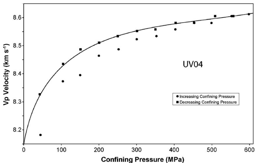
Fig. 4. Compressional wave velocity versus increasing and decreasing confining pressure for sample UV04. Velocities increase rapidly with increasing confining pressure as microcracks are closed. A least squares best-fit line is displayed through decreasing confining pressure points (see text for discussion). Some hysteresis is observed due to some microcracks staying closed as pressure is reduced.
