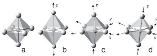
FIGURE 4. Different types of octahedral distortions: a = no distortion (cubic TiO), b = tetragonal distortion (rutile), c = trigonal distortion ( Ti_2O_3 ), d = orthorhombic-like distortion ( Ti_4O_7 and Ti_5O_9 ).
