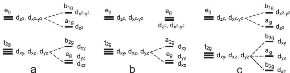
FIGURE 9. Splitting of the t_{2g} and e_g levels in tetragonal (a), trigonal (b), and orthorhombic (c) distorted environments.
