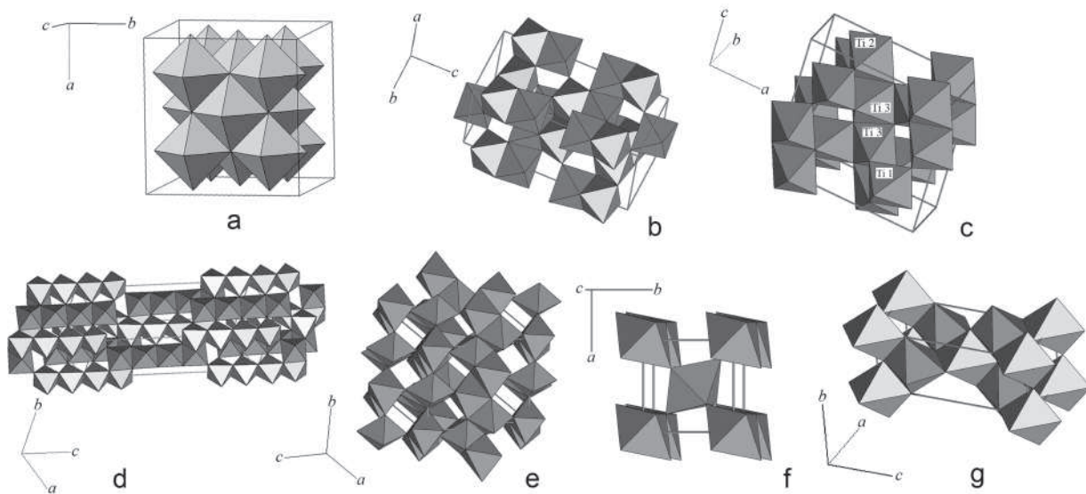
FIGURE 2. Crystal structures of the analyzed oxides: a = TiO ( Fm\bar{3}m ), b = Ti_2O_3 ( R\bar{3}c ), c = Ti_3O_5 ( C2/m ); d = Ti_4O_7 ( I\bar{1} ); e = Ti_5O_9 ( P\bar{1} ), f = TiO_2 (rutile, P4_2/mnm ), g = TiO_2 (anatase, I4_1/amd ).
