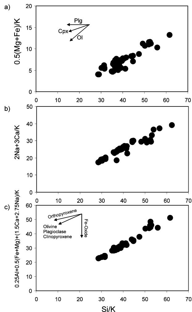
Figure 8. PER diagrams for the studied volcanics using K as a denominator. (a) 0.5(\text{Fe} + \text{Mg}) v. Si, (b) 2\text{Na} + 3\text{Ca} v. Si and (c) (0.25\text{Al} + 0.5(\text{Fe} + \text{Mg}) + 1.5\text{Ca} + 2.75\text{Na}) v. Si.
