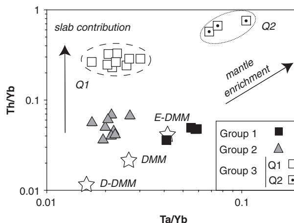
Fig. 8. Ta/Yb vs Th/Yb plot for primitive volcanic rocks from eastern Cuba (whole-rock analyses). Symbols as in Fig. 2. Open squares with dot, Quibjān 2 (Q2) volcanic rocks. DMM, D-DDM and E-DMM (stars) from Workman & Hart (2005). D, depleted; E, enriched.
