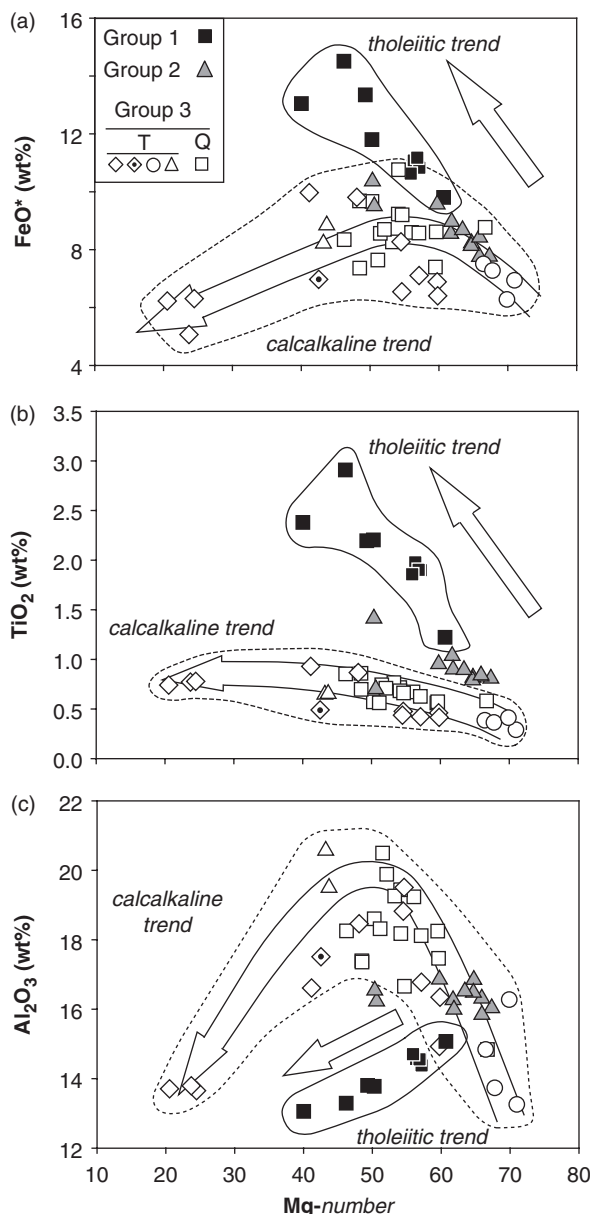
Fig. 3. Whole-rock major-element compositions of igneous rocks from eastern Cuba illustrated by Mg-number vs \text{FeO}^* (a), \text{TiO}_2 (b) and \text{Al}_2\text{O}_3 (c). Data plotted on an anhydrous basis in wt%. Symbols as in Fig. 2. The Téneme intrusive sample not plotted in Fig. 2 has been included here (open diamond with dot). Tholeiitic and calcalkaline differentiation trends marked by continuous and dashed lines, respectively.
