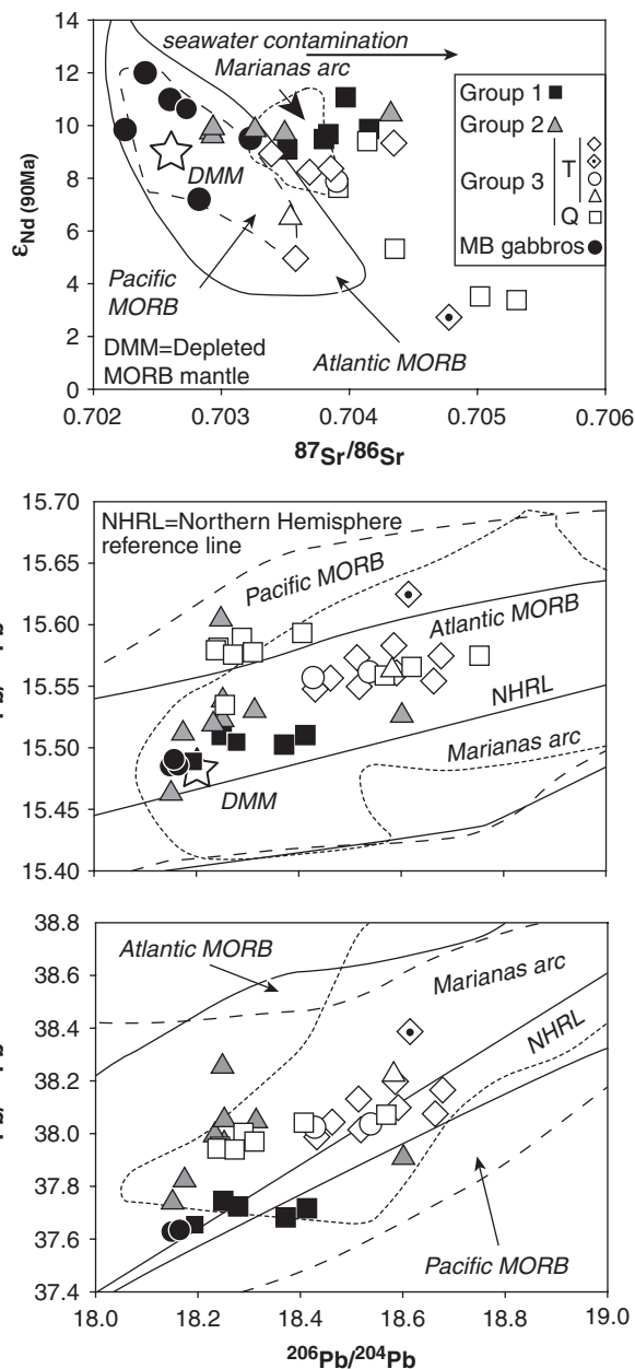
Fig. 6. Nd, Sr and Pb isotope ratios of whole-rocks and mineral separates for igneous rocks from eastern Cuba. For samples with known Rb, Sm, Th and U contents the data have been corrected for time-integrated radioactive decay since 90 Ma, according to the crystallization ages assigned by Iturralde-Vinent et al. (2006); otherwise, maximum present-day age-uncorrected values have been plotted. Symbols as in Fig. 3. ●, cumulate gabbros from the Moa–Baracoa (MB) ophiolitic massif. Depleted MORB mantle (DMM; star) from Workman & Hart (2005); Atlantic (continuous line) and Pacific (long dashed line) MORB fields from Hofmann (2003) and references therein; Marianas arc volcanic rocks field (short dashed line) from the GEOROC database ( http://georoc.mpch-mainz.gwdg.de/georoc/Entry.html ); NHRL (Northern Hemisphere reference line) from Hart (1984).
