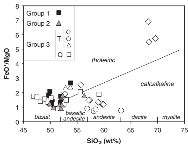
Fig. 2. \text{SiO}_2 vs \text{FeO}^*/\text{MgO} for volcanic rocks and dykes from eastern Cuba showing the discriminant boundary between tholeiitic and calcalkaline magmatic suites (Miyashiro, 1974). Data plotted on an anhydrous basis in wt%. \text{FeO}^* is total Fe as FeO. ■, Group 1 volcanic rocks; ▲, Group 2 dykes; ◇, Téneme volcanic rocks (Group 3T); ○, Téneme boninites (Group 3T); △, Estrella de Mayarí dykes (Group 3T); □, Quibiján volcanic rocks (Group 3Q). One dyke of Group 2 (LB 204) is not plotted because its whole-rock composition reflects significant amphibole accumulation.
