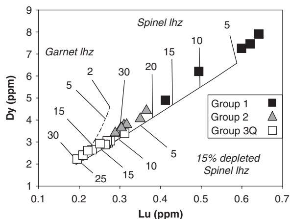
Fig. 7. Lu vs Dy (ppm) for primitive volcanic rocks (Mg-number >50; \text{SiO}_2 < 53 \text{ wt}\% ) from eastern Cuba (whole-rock analyses). Symbols as in Fig. 2. Non-modal batch melting curves are labelled for variable melting degrees of spinel lherzolite (lh) (continuous line) [source and melting ol:opx:cpx proportions 0.57:0.28:0.15 and 0.13:0.27:1.4, respectively (Walter et al. , 1995)] and garnet lherzolite (dashed line) [source and melting ol:opx:cpx:grr proportions 0.52:0.29:0.16:0.03 and 0.0:45:0.45:0.1, respectively (Gribble et al. , 1998)] with depleted composition (Donnelly et al. , 2004). Partition coefficients from Bedini & Bodinier (1999), Su & Langmuir (2003) and Donnelly et al. (2004).
