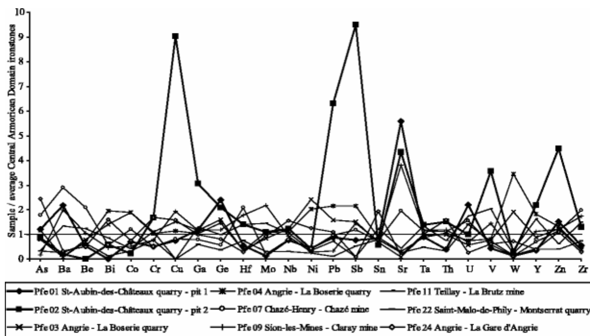
Fig. 7 Comparison of the trace element composition of regional A-layer ironstone with the non-altered (Pfe 01) and hydrothermally altered (Pfe 02) samples from the Saint-Aubin-des-Châteaux quarry. All samples are normalised to the average regional ironstone composition (Table 1)
