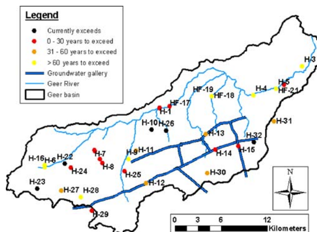
Fig. 8 Time (years) foreseen before the 50 mg/L \text{NO}_3^- threshold will be exceeded in groundwater
