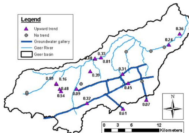
Fig. 7 Spatial distribution of nitrate trends in the Geer basin groundwater, with nitrate upward trend values in mg/L \text{NO}_3^- per year
