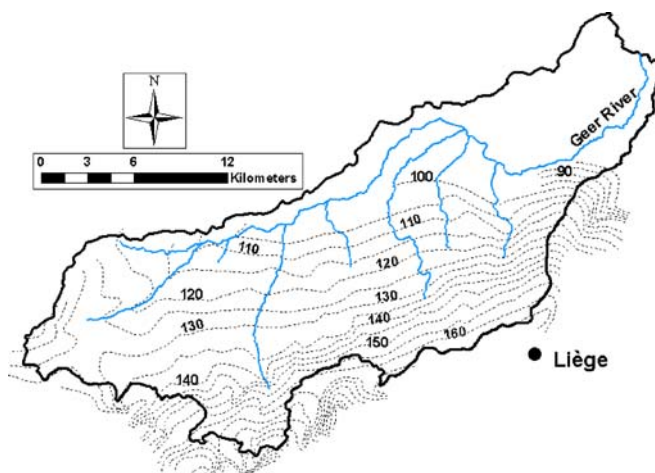
Fig. 4 Piezometric map of the Geer basin, based on a groundwater survey campaign in 1984 on the Hesbaye aquifer (in metres asl)
